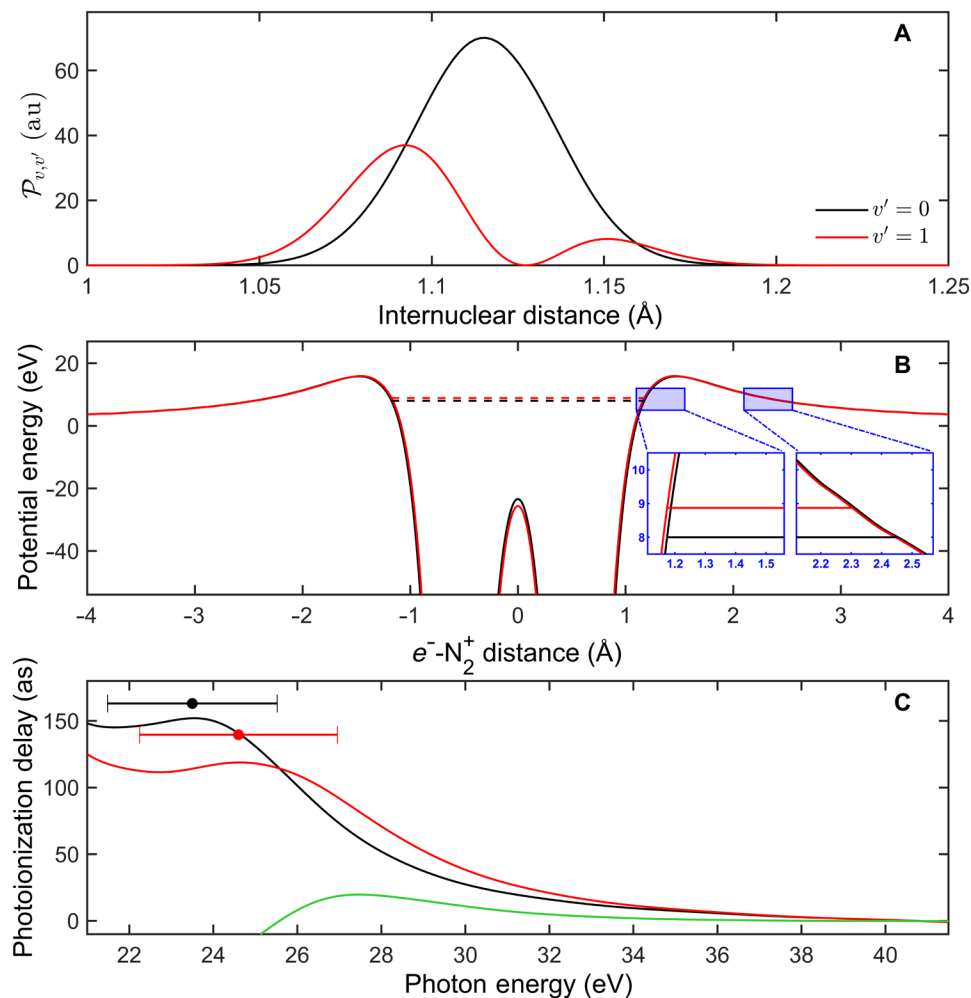
Fig. 5. Electron dynamics induced by structural changes. (A) Absolute square of the transition matrix element d_{\sigma_u, \sigma_g}^X at an electron kinetic energy of 8.2 eV, multiplied by the initial ( \chi_{i,v=0} ) and final ( \chi_{f,v'} ) vibrational wave functions, \mathcal{P}_{v,v'} , as a function of the internuclear distance R . The red and black curves correspond to transitions from the v = 0 level in the neutral ground state to the v' = 1 and the v' = 0 levels of the X state, respectively. (B) Potential felt by an electron escaping from an N 2 molecule with internuclear distance R_{v=1} = 1.09 Å (red) and R_{v=0} = 1.113 Å (black), calculated at the same level of theory as the dipole matrix elements. These Kohn-Sham potentials are shown along the internuclear axis, with the two wells representing the two N atoms. The origin is placed at the center of mass of the molecular ion. The dashed lines show the corresponding resonance energies. As shown in the insets, the barrier width depends on R , hence, on the vibrational state of the ion. Figure 5C shows the photoionization delays ( \tau_1 ) as a function of photon energy obtained at the internuclear distances R_{v=1} = 1.09 Å (red) and R_{v=0} = 1.113 Å (black) and the relative delay between them, \tau_1^X(R_{v=1}) - \tau_1^X(R_{v=0}) (green). The resonance lifetimes (full circles) and widths (horizontal bar) calculated in the Wentzel-Kramers-Brillouin (WKB) approximation from the two potentials presented in Fig. 5B are also shown.
