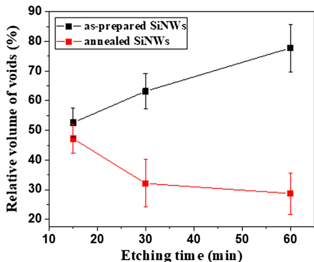
Fig. 3. Relative volume of voids versus etching time for SiNWs arrays before (black squares) and after (red squares) TA treatment.
