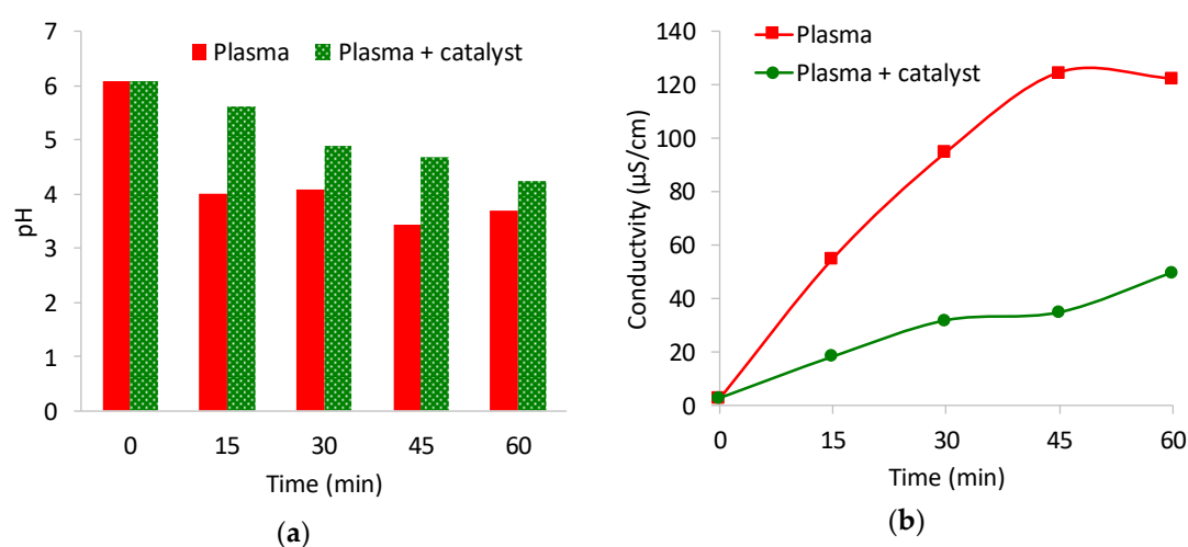
Figure 9. pH (a) and conductivity values (b) of the solutions treated by NTP/Fenton-like coupling compared to those with NTP alone ( U = \pm 5.9 kV, f = 500 Hz, electrode-liquid-gap = 5 mm, Q_{\text{air}} = 100 sccm, [Paracetamol] = 25 mg L -1 , V = 40 mL, \text{pH}_0 = 6.1 , \sigma_0 = 2.61 μS·cm -1 ).
