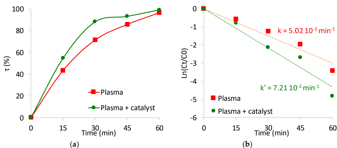
Figure 2. (a) Conversion rates (mean values of 3 runs for each operating condition) of paracetamol treatment as a function of treatment time and (b) kinetics of paracetamol degradation by NTP without and with catalysis coupling ( U = \pm 5.9 kV, f = 500 Hz, electrode-liquid-gap = 5 mm, Q_{\text{air}} = 100 sccm, [\text{Paracetamol}] = 25 \text{ mg L}^{-1} , V = 40 \text{ mL} ).
