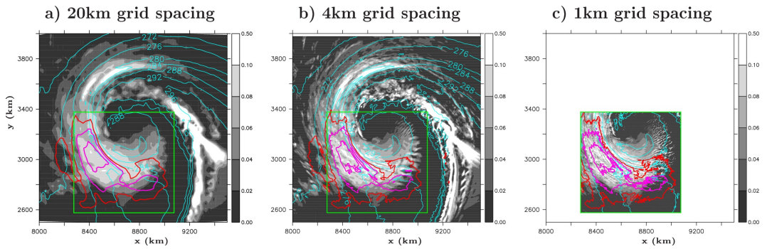
FIGURE 2 Maximum of the sum of cloud liquid and ice water contents between z = 0.5 km and z = 2.0 km (grey shadings; units: \text{g kg}^{-1} ), horizontal wind speed at z = 1.6 km ( 30 \text{ m s}^{-1} in red and 35 and 40 \text{ m s}^{-1} in magenta), and equivalent potential temperature at z = 1.6 km (light blue contours; interval: 4 K) at t = 93 h for different simulations: (a) S20land, (b) S4land and (c) S1land.
