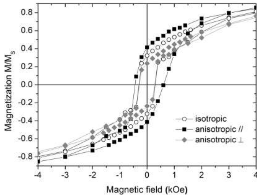
Figure 5: Magnetization of composites with isotropic fibers orientation (white circle), and with aligned fibers, measured along the fiber (black square) and perpendicular to the fiber (grey diamond).
