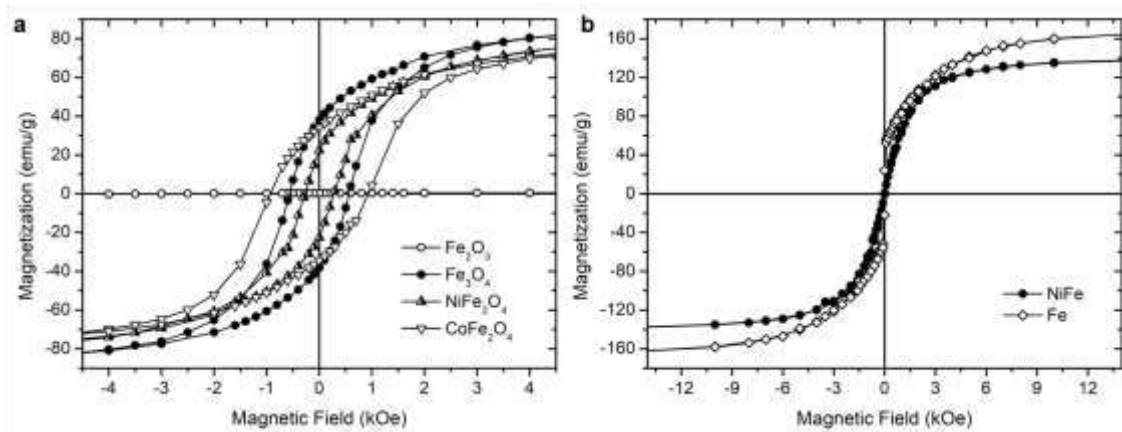
Figure 3: Room temperature magnetization curves of fibers: (a) Fe_3O_4 , Fe_2O_3 , CoFe_2O_4 , NiFe_2O_4 , (b) Fe , NiFe .
