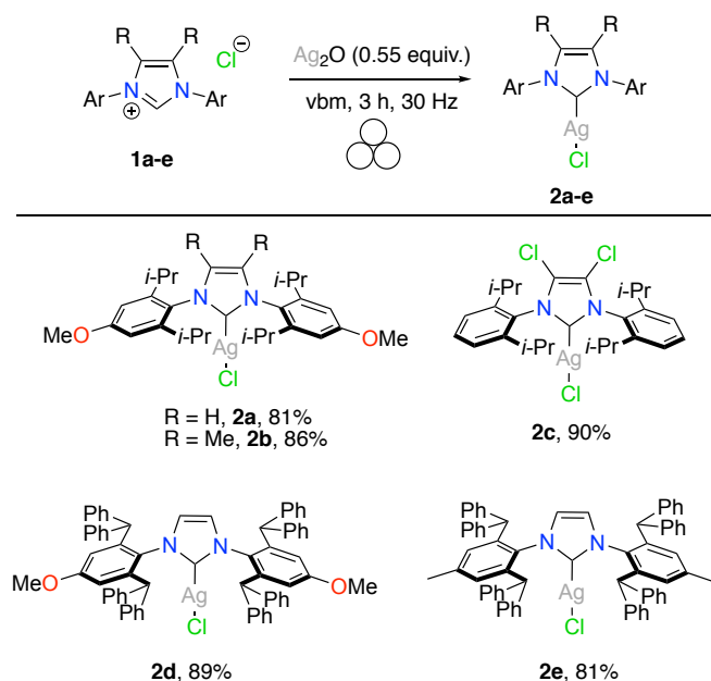
Scheme 1. Mechanochemistry of [\text{AgCl}(\text{NHC})] complexes bearing highly encumbered NHC ligands
