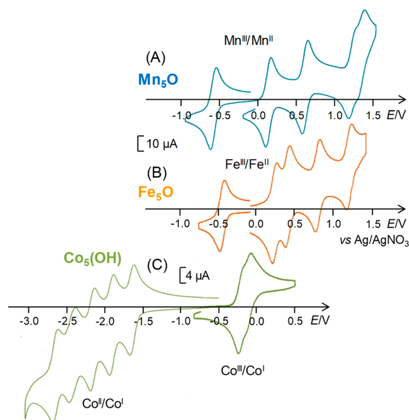
Figure 3. Cyclic voltammograms in \text{CH}_3\text{CN} and 0.05 M [\text{Bu}_4\text{N}]\text{ClO}_4 of (A) a 0.7 mM solution of [\{\text{Mn}^{\text{II}}(\mu\text{-bpp})_3\}_2\text{Mn}^{\text{II}}\text{Mn}^{\text{III}}(\mu_3\text{-O})]^{3+} at a Pt electrode (diameter of 5 mm), (B) a 0.5 mM solution of [\{\text{Fe}^{\text{II}}(\mu\text{-bpp})_3\}_2\text{Fe}^{\text{II}}\text{Fe}^{\text{III}}(\mu_3\text{-O})]^{3+} at a Pt electrode (diameter of 5 mm), and (C) a solution of [\{\text{Co}^{\text{II}}(\mu\text{-bpp})_3\}_2\text{Co}^{\text{II}}(\mu_3\text{-OH})]^{3+} ( \text{I}^{3+} ) at a Pt electrode (diameter of 3 mm) with a scan rate of 100 \text{mV s}^{-1} .
