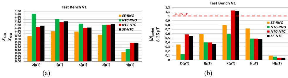
Figure 16. Comparison of values of |B| levels of interoperability prototypes (a) simulation results normalized to test ones and (b) tests results normalized to 6.25 \mu T.
