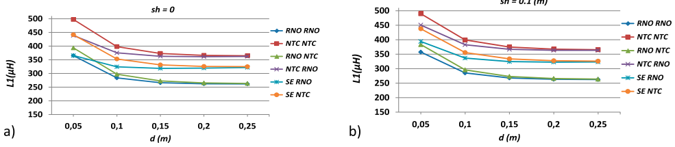
Figure 11. Values of L_1 for different prototypes as a function of the air gap distance d(m) : (a) sh = 0 and (b) sh = 0.1 m.
