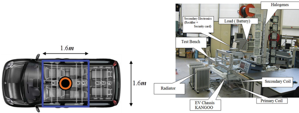
Figure 7. Experimental validation with a chassis of Renault KANGOO.
