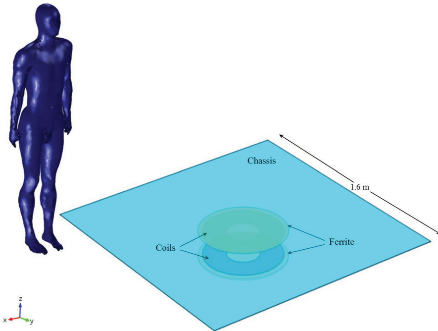
Figure 17. Human body model and representative wireless inductive charging system.
