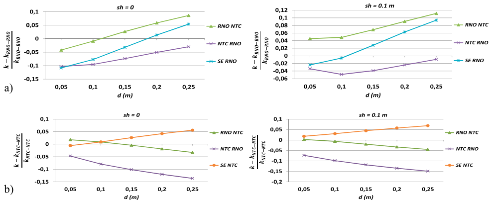
Figure 15. Comparison of relative difference of the coupling factor for two groups of reference prototype: (a) k_{ref} : RNO-RNO and (b) k_{ref} : NTC-NTC.
