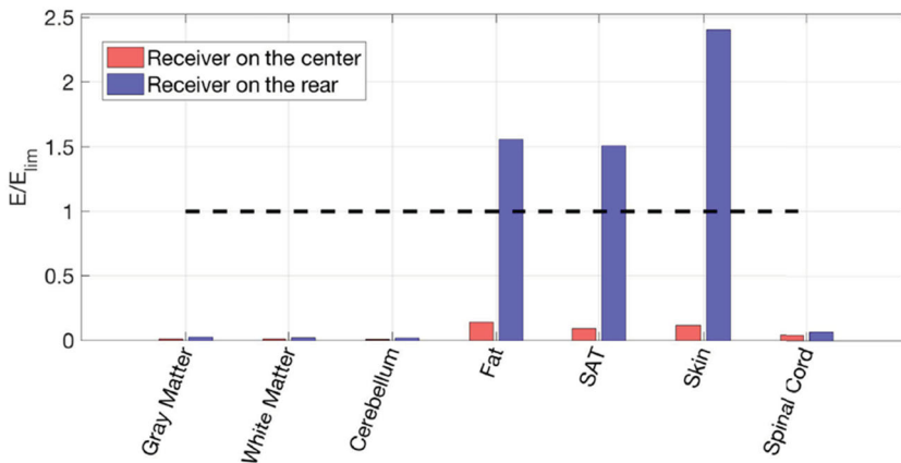
Figure 21. Exposure index on the selected tissues for the analyzed worst cases.
