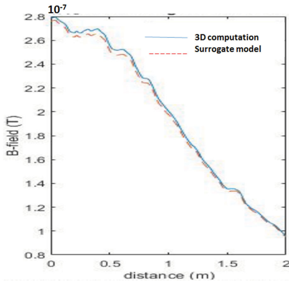
Figure 29. B-field on a vertical line located at 1.5 m from the side of the vehicle.
