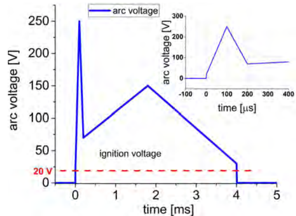
Fig. 16. Time behavior of the simulated arc voltage.
