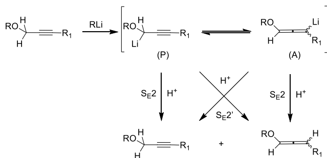
Scheme 2. Metallotropic equilibrium between generally proposed Li-propargyl and Li-allenyl intermediates and protonation pathways.
