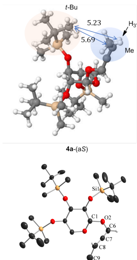
Figure 1. Above: Optimized structure of the major diastereoisomer 4a -(aS) with OTBS groups in axial position obtained by DFT calculations (B3P86/6-31+G(d,p) level) showing the distances (in Å) between H 3 ' and methyl group on allene with OTBS group. Below: Crystal structure of 4a -(aS) with OTBS groups in equatorial position. Ellipsoids are represented at 30 % probability; hydrogen atoms are omitted for clarity, except for the allene hydrogens.
