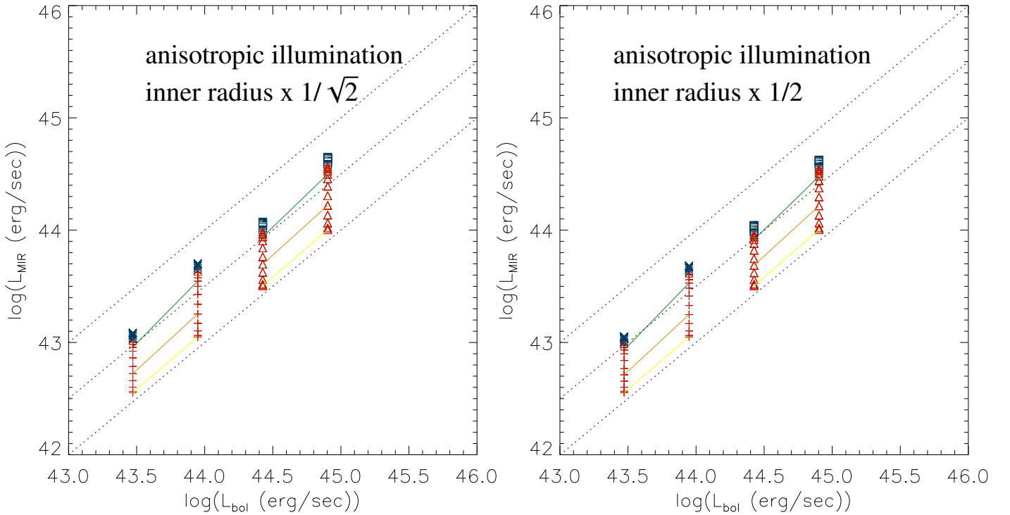
Fig. 15. Model MIR luminosities as a function of the bolometric luminosity for the 1/z winds with anisotropic illumination for a \sqrt{2} (left panel) and 2 (right panel) times smaller inner radius of the thin gas disk. The dotted lines correspond to L_{\text{MIR}} = \xi L_{\text{bol}} with \xi = 1, 1/3 , and 1/10 .
