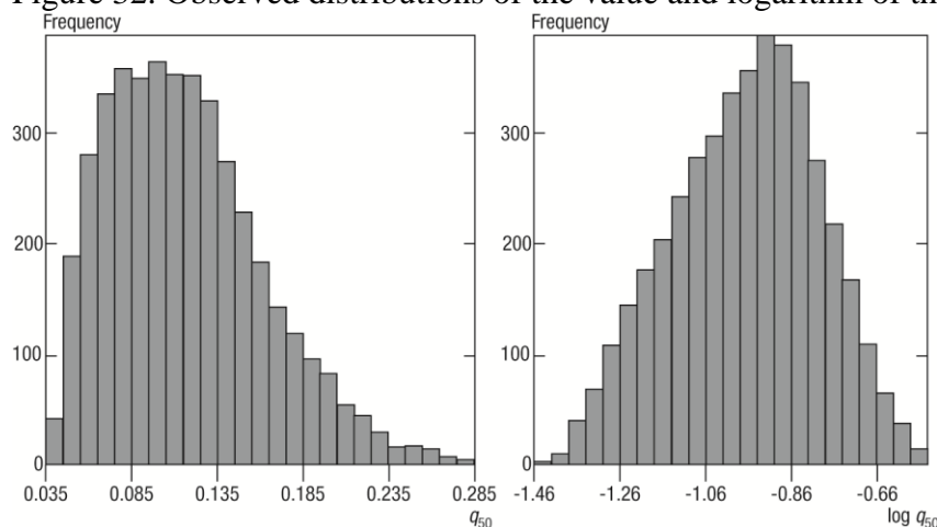
Figure 32. Observed distributions of the value and logarithm of the probability of dying q_{50}
