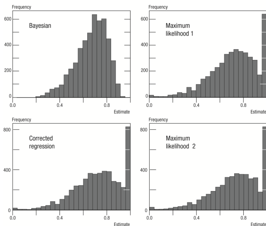
Figure 70. Simulations – Example 2: histograms of estimates obtained by four methods (with \beta_1 = \beta_2 = 1 for the Bayesian method)
