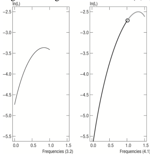
Figure 68. Log-likelihood for x = (3, 2) , left, and \xi = (4, 1) , right
