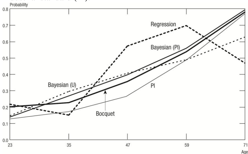
Figure 76. Probabilities of death for Loisy-en-Brie estimated by the Bayesian method with pre-industrial standard prior (Bayesian PI), uniform prior (Bayesian U), regression, and the method proposed by Bocquet-Appel and Bacro in 2008 (Bocquet), compared with the pre-industrial standard (PI).
