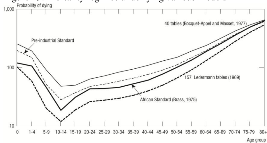
Figure 29. Mortality regimes underlying various models
