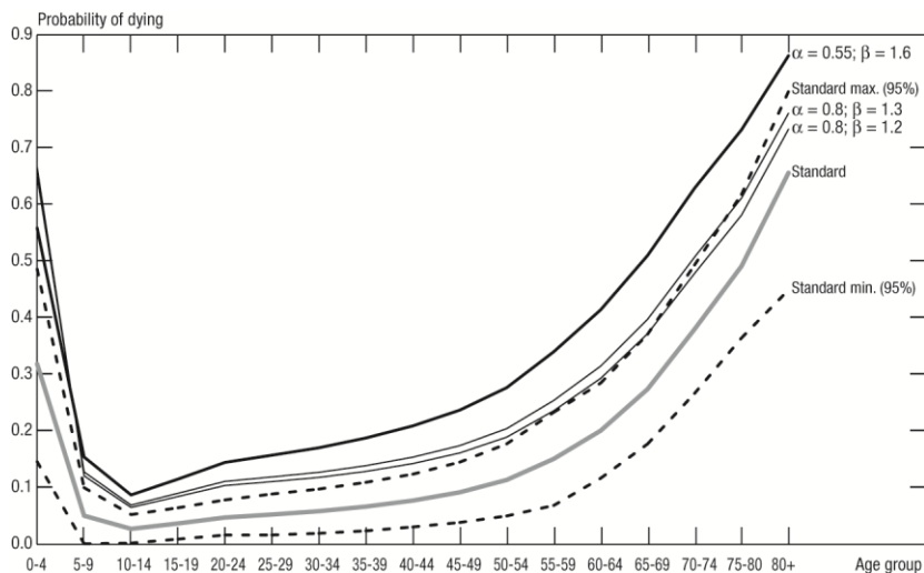
Figure 47. Probabilities of dying by age associated with various combinations of model parameters \alpha and \beta , such that the juvenility index exceeds 0.245.
