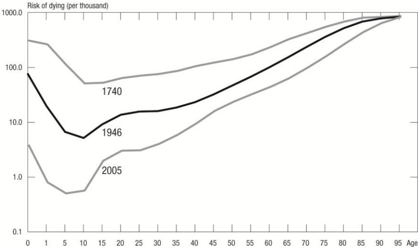
Figure 27. Risk of dying at a given age in France, 1740-2005 (both sexes)
