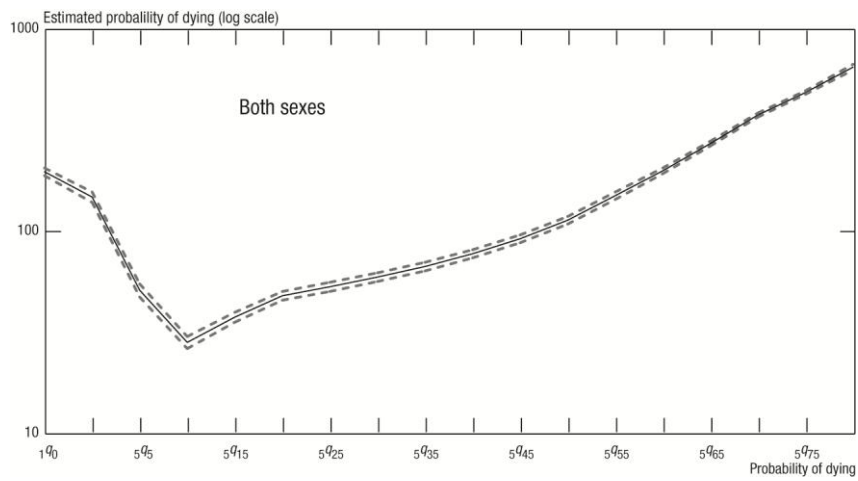
Figures 35, 36, 37. Pre-industrial standard: probability of dying by age
