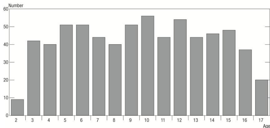
Figure 25. Age distribution of the sample of orthopantomograms
