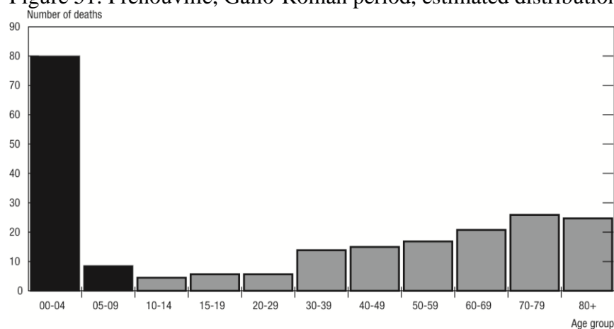
Figure 51. Frénouville, Gallo-Roman period, estimated distribution of deaths by age group
