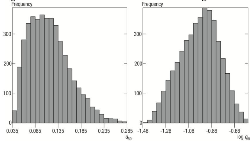
Figure 32. Observed distributions of the value and logarithm of the probability of dying q_{50}
