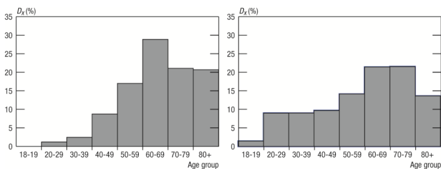
Figure 57. Theoretical distribution of deaths by age
