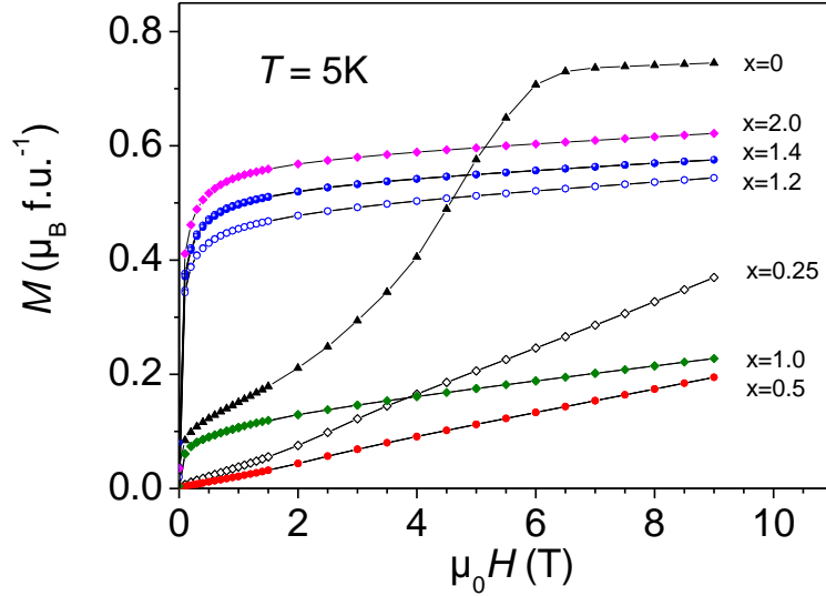
Figure 6. Magnetization curves of \text{La}_{2-x}\text{Y}_x\text{Ni}_7 compounds versus applied field at 5 K.
