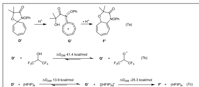
Scheme 7 Computed protonation of the spiro intermediate D' and deprotonation of G' .
