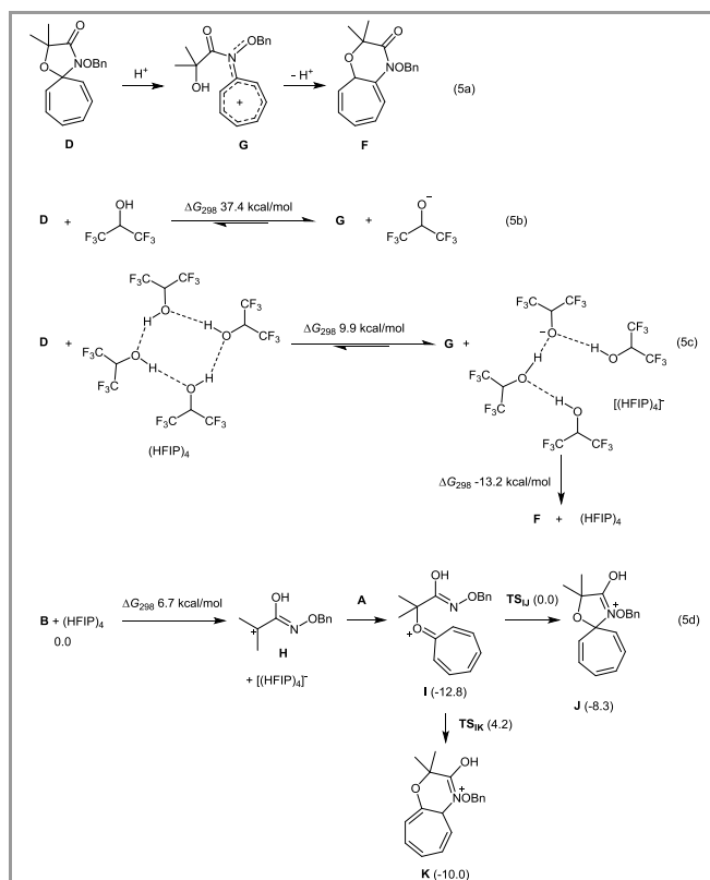
Scheme 5 Computed protonation of intermediates D and B .
