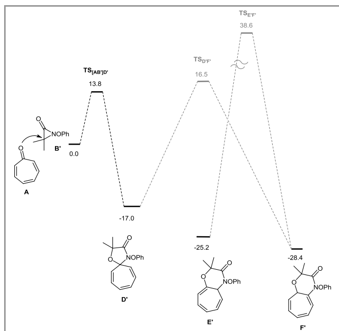
Scheme 6 Computed free energy profile using the phenyl-substituted intermediate B' ( \Delta G_{298} , kcal/mol).
