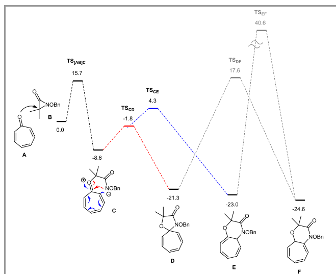
Scheme 4 Computed free energy profile using the benzyl-substituted intermediate B ( \Delta G_{298} , kcal/mol).
