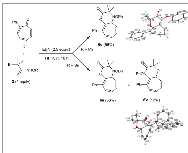
Scheme 2 Influence of tropone substitution on the reactivity. ORTEP drawings of compounds 6e and 6'a . Thermal ellipsoids are shown at 30% probability level.
