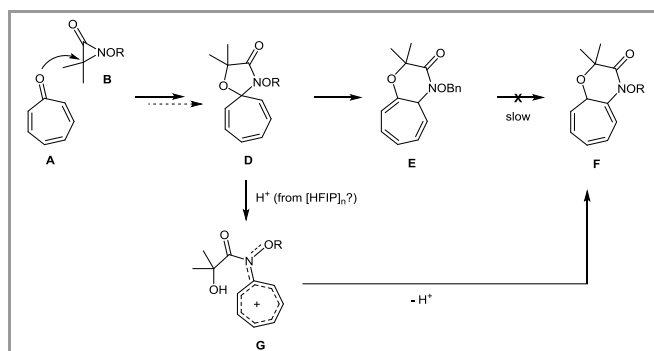
Scheme 8 Plausible mechanism
