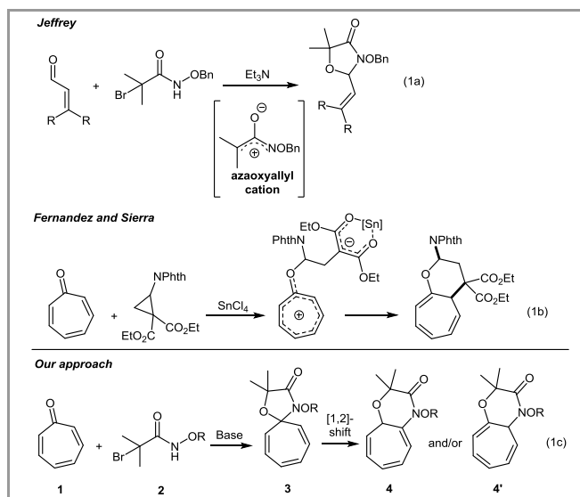
Scheme 1 [8+3] annulation between tropone and azaoxyallyl cation
