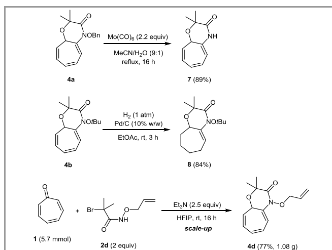
Scheme 3 Post-modifications and scale-up
