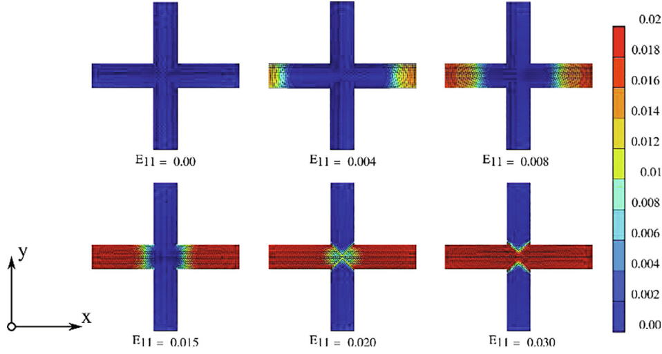
Fig. 8. Accumulated plastic strain map in the square lattice 0°-oriented unit cell.
