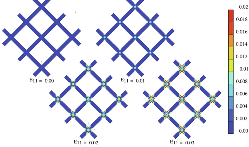
Fig. 13. Plastic strain map in a 9-cell 45°-oriented square lattice.
