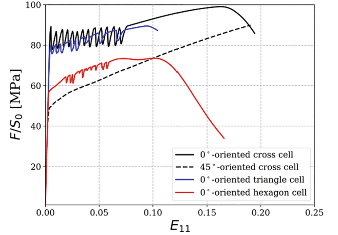
Fig. 28. Simulation of the architected samples: stress-strain curves.
