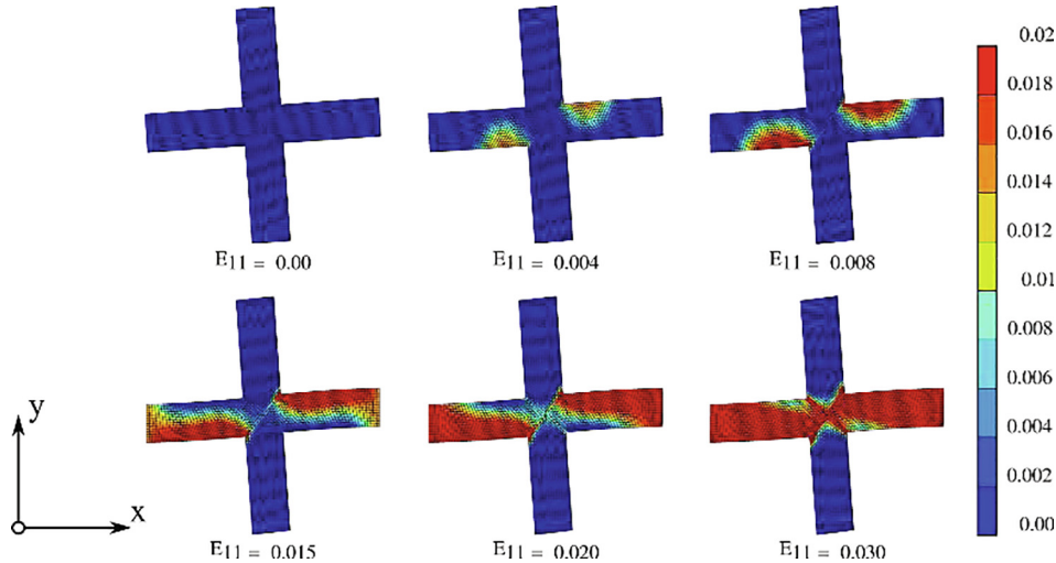
Fig. 9. Accumulated plastic strain map in the square lattice 4°-oriented unit cell.
