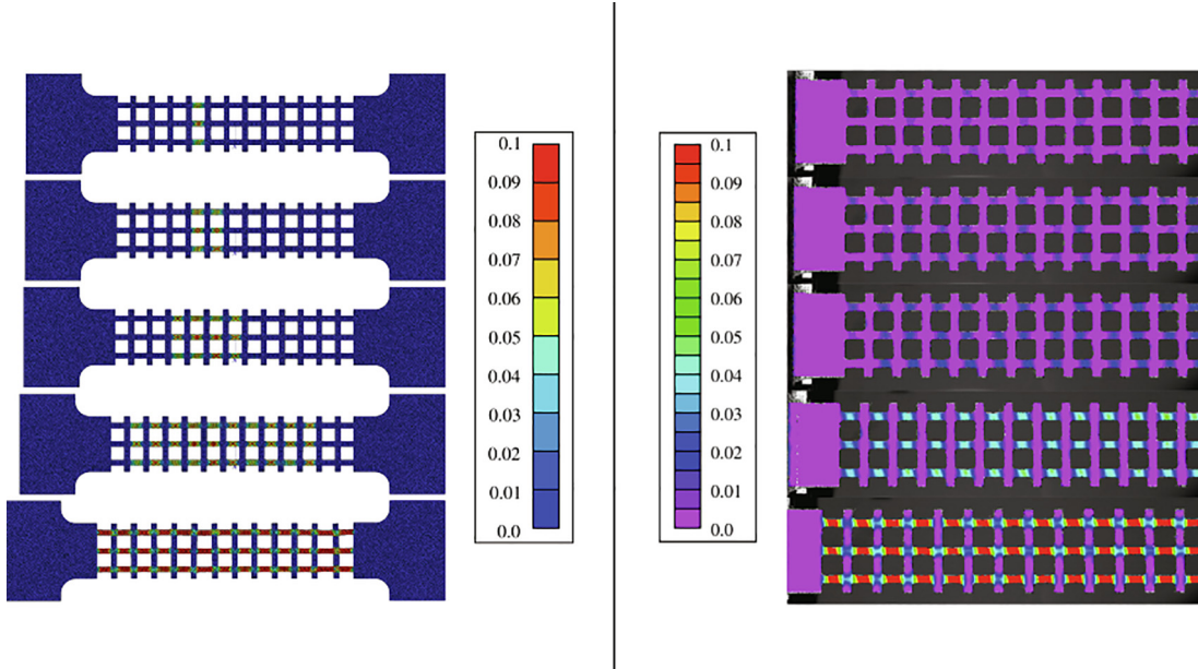
Fig. 29. e_1 strain map in the tensile direction for the 0^\circ -oriented square lattice with comparison of the simulation on the left to the experiment on the right.
