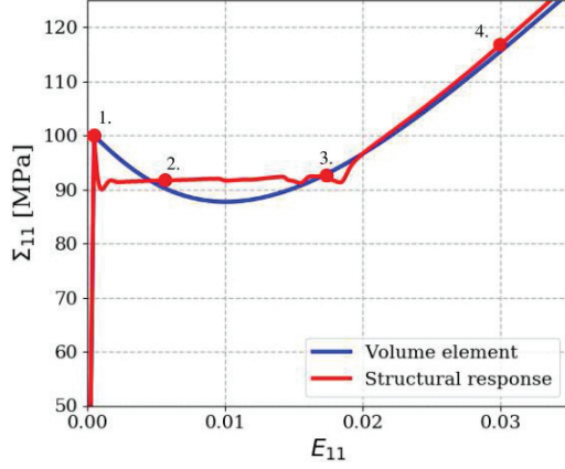
Fig. 3: Intrinsic constitutive law for Lüders phenomenon integrated on a single Gauss point (Volume element) compared to the overall response of a plate endowed with this material behavior. The accumulated plastic strain maps corresponding to the points (1,2,3,4) marked on the plate response curve are shown in Figure 4.
