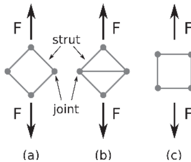
Fig. 1: (a) a mechanism; (b) a structure; (c) self-stressed state mechanism adapted from Deshpande et al. (2001)
