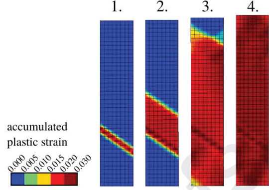
Fig. 4: Accumulated plastic strain map on a sample in tension with propagation of a Lüders localization band.
