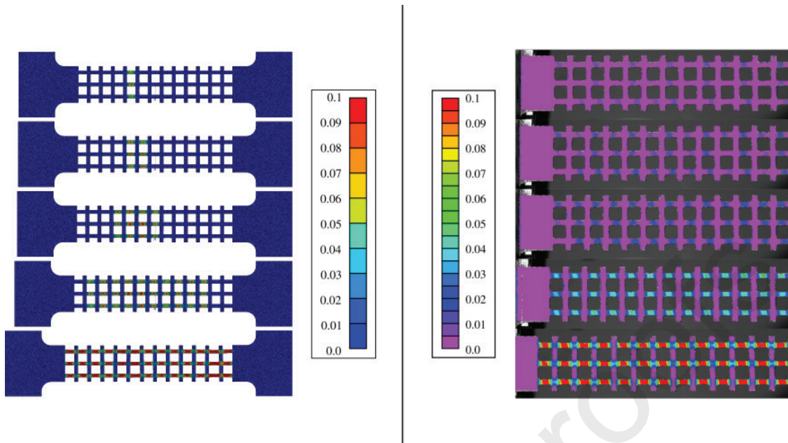
Fig. 29: \epsilon_1 strain map in the tensile direction for the 0°-oriented square lattice with comparison of the simulation on the left to the experiment on the right.
