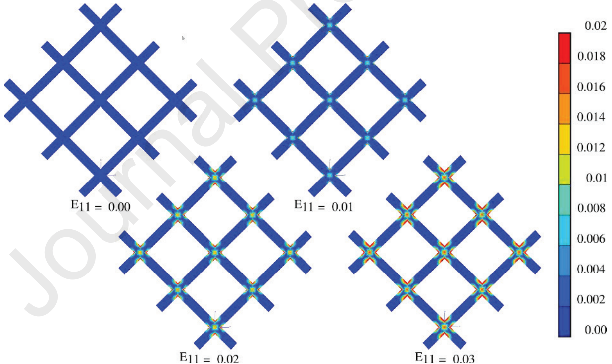
Fig. 13: Plastic strain map in a 9-cell 45^\circ -oriented square lattice.
