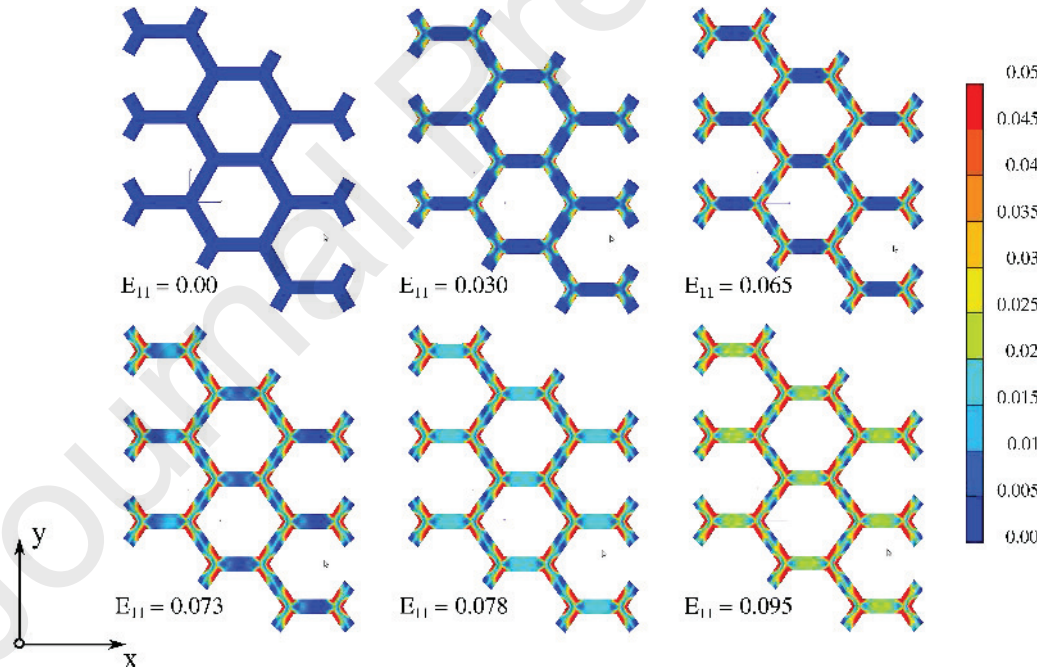
Fig. 19: Plastic strain map in a 9-cell 0^\circ -oriented hexagonal lattice.
