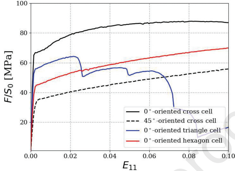
Fig. 25: Experimental stress-strain curves of architected samples.
