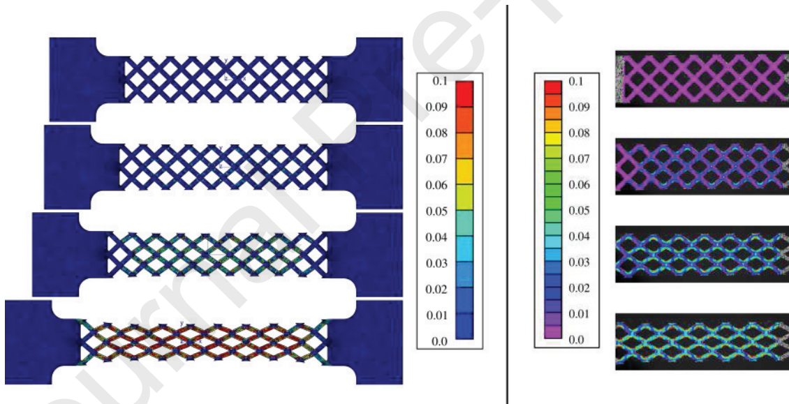
Fig. 30: \epsilon_1 strain map in the tensile direction for the 45°-oriented square cell with comparison of the simulation on the left to the experiment on the right.
