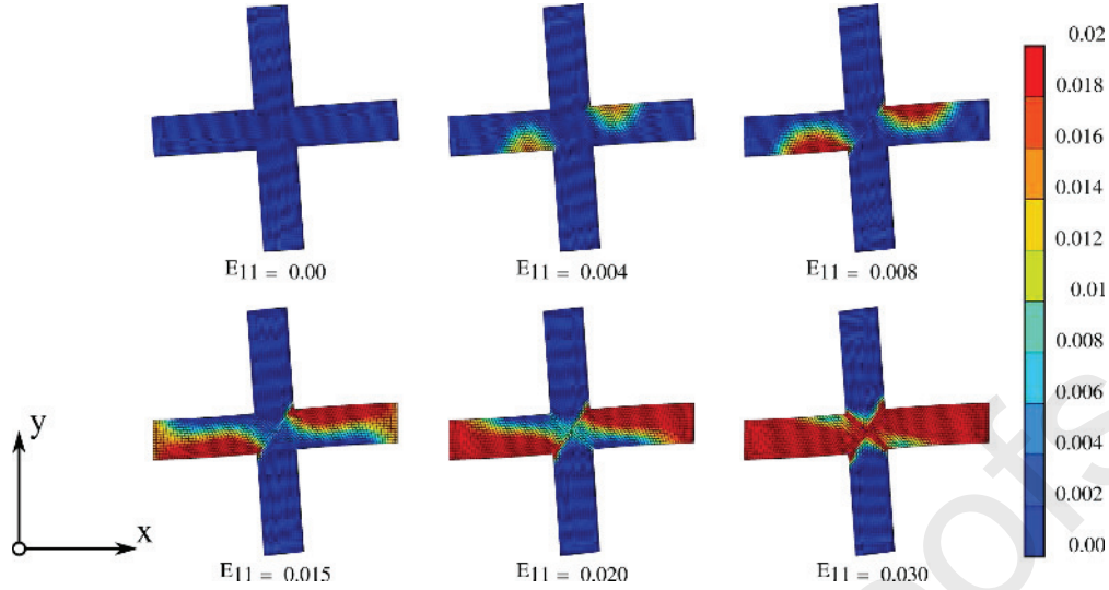
Fig. 9: Accumulated plastic strain map in the square lattice 4^\circ -oriented unit cell.
