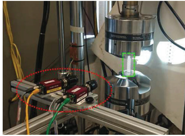
Fig. 22: Experimental set-up for digital image correlation. In red: cameras system, in green: tensile specimen.
