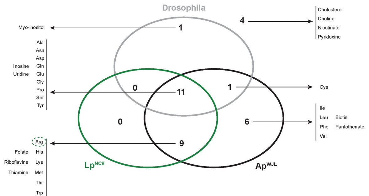
Fig 2. Drosophila , Ap^{WJL} , and Lp^{NC8} have differential biosynthetic capacities of nutrients contained in the HD. Venn diagram represents the number of nutrients present in the FLYAA HD that can be synthesized by each organism. The list of corresponding metabolites is provided. Dotted circles: biosynthesis of this metabolite by Lp^{NC8} (green) may be possible but might be limiting. Ap^{WJL} , A. pomorum WJL ; FLYAA, fly exome-matched amino acid ratio; HD, Holidic Diet; Lp^{NC8} , L. plantarum NC8 .
