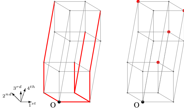
Figure 2: The up-oriented paths of length 3 in the hypergrid H_{4,1} and their final vertices.
