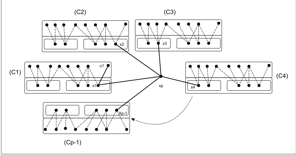
Fig. 5: An example when G' is a star.
