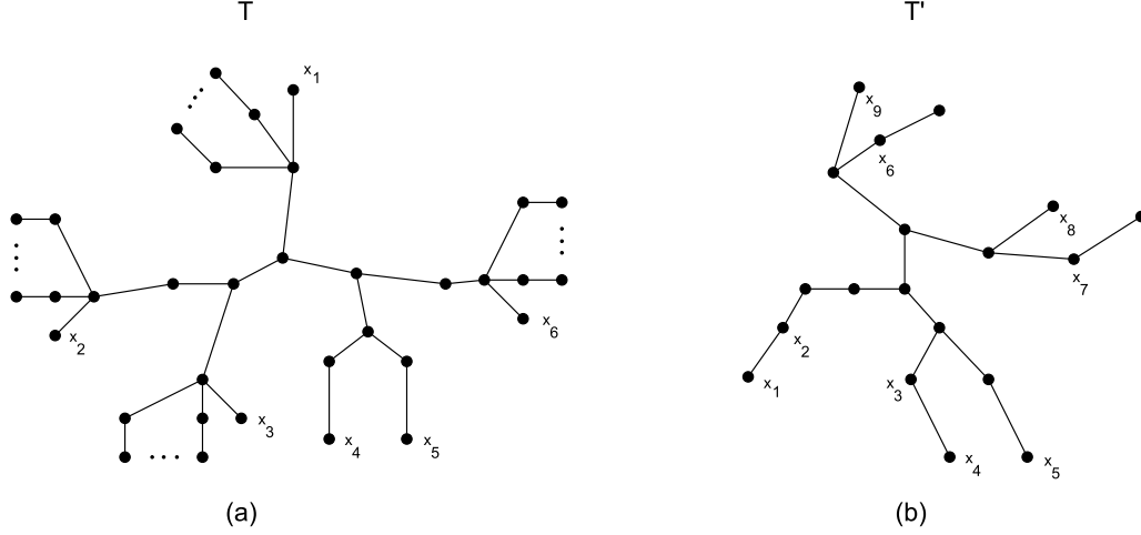
Figure 1: (a) T is (-6) -critical and \sigma(T) = \{x_1, \dots, x_6\} . (b) T' is minimal for \{x_1, \dots, x_9\} .
