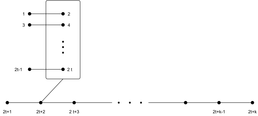
Figure 3: The tree P_{k,t}
