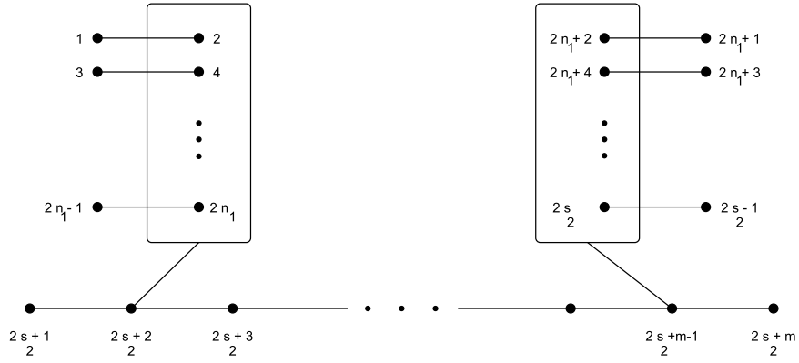
Figure 4: The tree P_{m,n_1,n_2}
