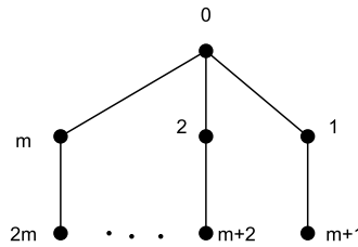
Figure 2: The tree A_{2m+1}
