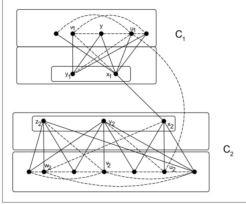
Fig. 4: Illustration of Lemma 3.2. The dots edges are in the second copy of G .
