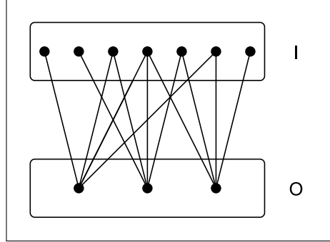
Fig. 1: A B_{IO} – graph with 10 vertices.
