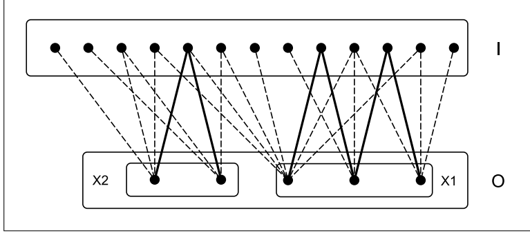
Fig. 2: An example of a partition \mathcal{P}(O) .
