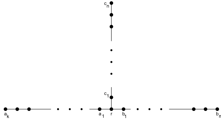
Figure 5: S_{k,m,n}
