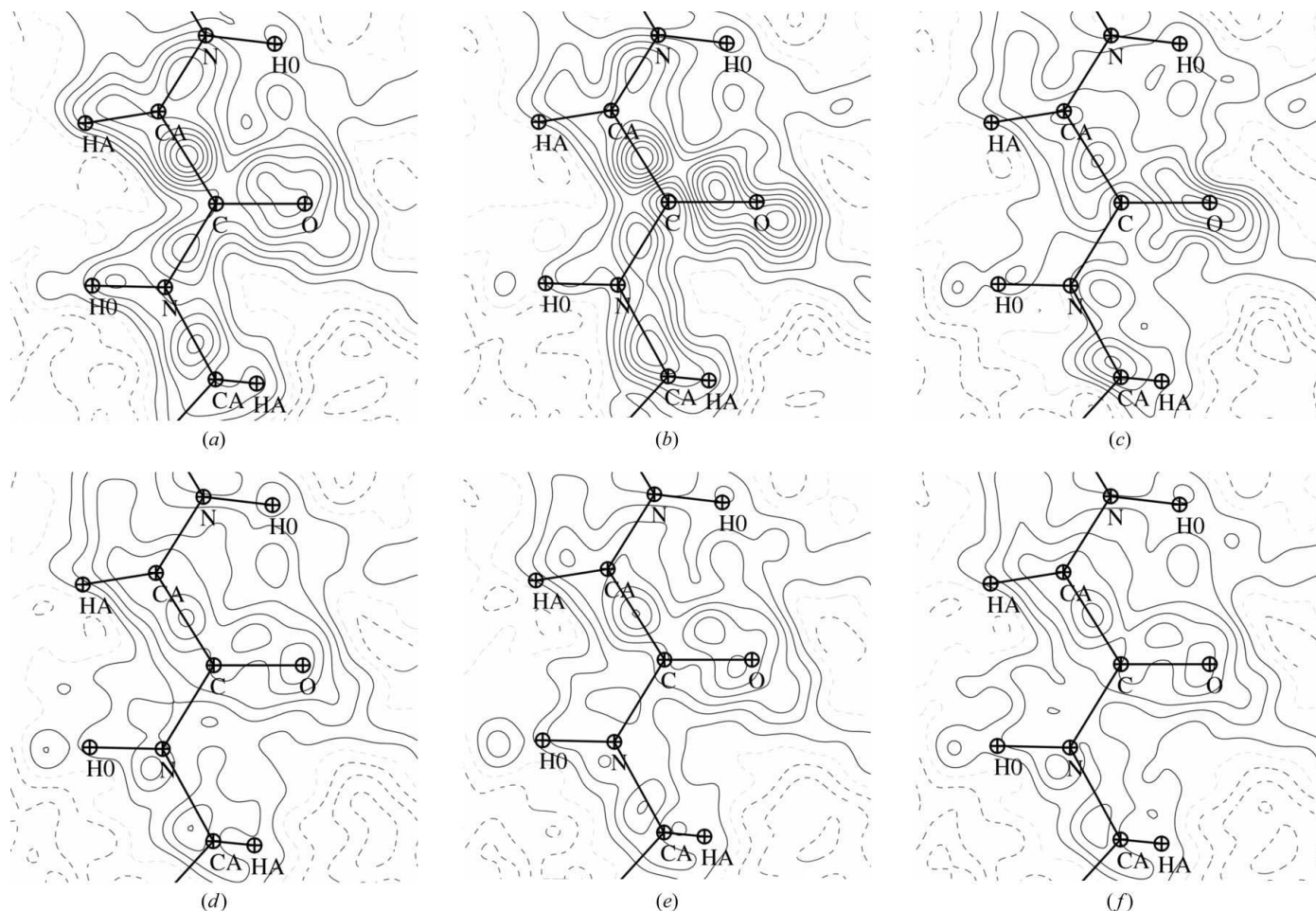
Figure 11 Evolution of residual electron density on the Ala45–His46 peptide bonds of the substructure during the various refinement steps. The stages of refinement are (a) IAM unrestrained, (b) IAM HO, (c) after database-transfer procedure, (d) after positional and thermal motion parameter refinement to readjust the transfer, (e) after IAM multipolar refinement and (f) after ELMAM multipolar refinement. Contours are as in Fig. 6.
