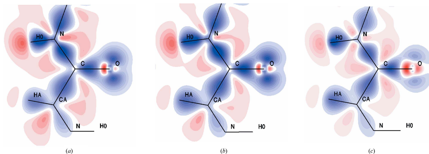
Figure 12 Static deformation electron density in the plane of the peptide bond. (a) As transferred from ELMAM library. (b) After ELMAM constrained multipolar refinement. (c) After multipolar refinement starting from IAM spherical neutral atoms. Contours are \pm 0.05 \text{ e } \text{Å}^{-3} , with positive values in blue and negative values in red. Electron-density values between -0.05 and +0.05 \text{ e } \text{Å}^{-3} are not represented.
