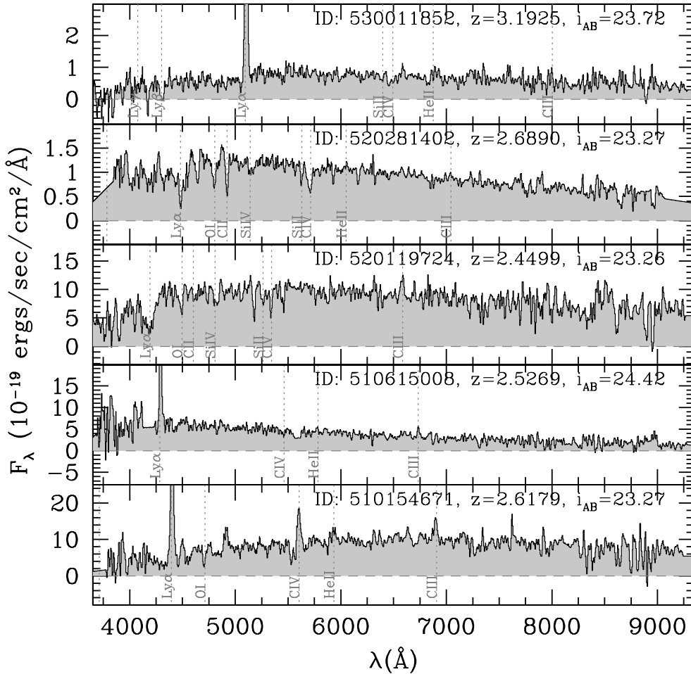
Fig. 3. Example VUDS spectra of weak CIII]1908 emitters with 0 < EW(CIII)] < 5 Å.
