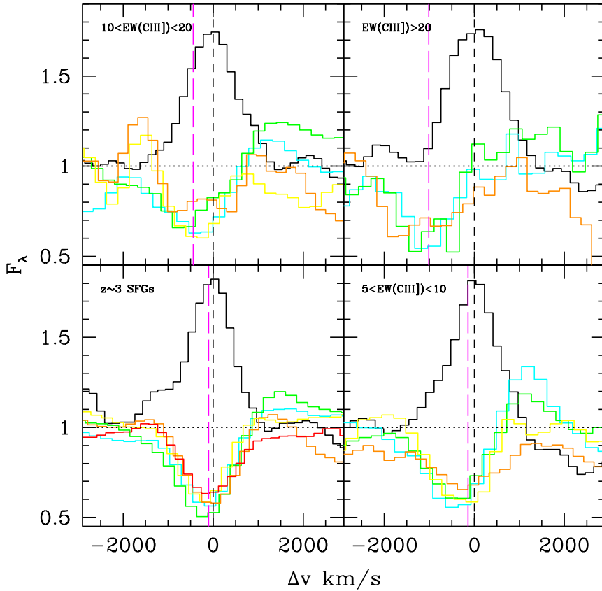
Fig. 9. Relative velocity of the main ISM absorption lines with respect to CIII]- \lambda 1908 Å taken as systemic velocity for the SFG population and samples with increasing EW(CIII)]. CIII] is plotted in black, and depending on the sample, SiII- \lambda 1260 is drawn in cyan, SiII- \lambda 1303 in green, CII- \lambda 1334 in yellow, 1526 in orange, and 1670 in red. The mean outflow velocities (see text) are indicated as the long-dashed magenta lines.
