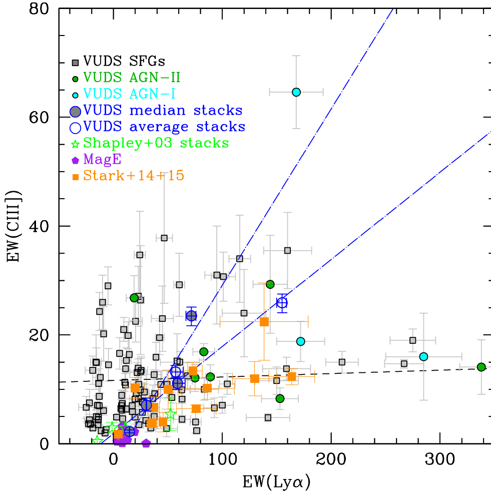
Fig. 6. Rest-frame equivalent width of CIII]- \lambda 1908 EW(CIII]) as a function of EW(Ly\alpha) . The least-squares fit to the individual data points (black squares) is represented by the black dashed line. The individual galaxies show only a weak correlation that is significant at about the 3\sigma level, with a large dispersion. Galaxies with strong Ly\alpha and weak CIII] are observed, as well as galaxies with strong CIII] and Ly\alpha in absorption. The EW(CIII]) vs. EW(Ly\alpha) points for the median-stacked spectra of the different categories defined in Sect. 3 are indicated as blue circles filled with gray, while values for the average stacks in Table A.1 are indicated as open blue circles. The correlation between EW(CIII]) and EW(Ly\alpha) appears to be very strong ( r_p = 0.99 , r_s = 1 ) and hides the wide range of properties of CIII] vs. Ly\alpha . As a comparison with the literature, we plot the observed values from the different Ly\alpha samples of Shapley et al. (2003) (green stars, average for Ly\alpha samples), Rigby et al. (2015) (purple diamonds), and Stark et al. (2014, 2015) (orange squares).
