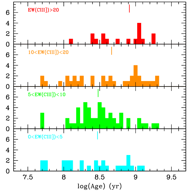
Fig. 13. Age distribution of CIII] emitters with different EW(CIII]). The median age of each population is identified by the color of the vertical lines as for their respective subsamples. The strength of the CIII] emission increases with mean age.
