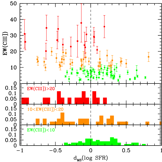
Fig. 12. Bottom three panels: distribution of distances in SFR from the main sequence for CIII] emitters with increasing EW(CIII]), and top panel: distance to the main sequence for individual CIII] emitters. As EW(CIII]) increases, the distance to the main sequence increases.
