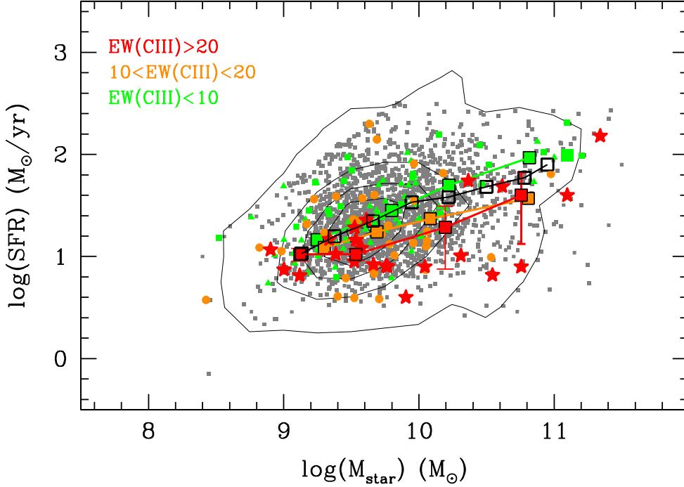
Fig. 11. Distribution of CIII] emitters with different EW(CIII]) in the M_{\text{star}} –SFR plane. The CIII] emitters with different EW are identified by the differently colored symbols. The parent sample of star-forming galaxies at redshifts 2 < z < 3.8 in VUDS is identified as gray symbols whose distribution is identified by the contours, and the main sequence of VUDS galaxies at z \sim 3 is indicated by black open squares that are connected by a thick line. We note that both the strong and very strong CIII] emitters are on average below the MS, with median values identified by the connected orange and red squares, respectively. The lower SFR of these strong CIII] emitters compared to the MS is possibly caused by a strong star formation quenching produced by AGN feedback in the host star-forming galaxies.
