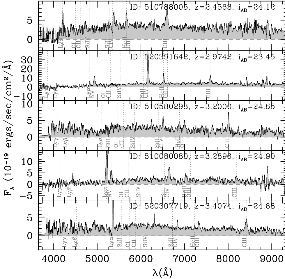
Fig. 1. Example VUDS spectra of CIII]1908 emitters with very strong \text{EW}(\text{CIII])} \geq 20 Å. The spectra of strong CIII] emitters are highly diverse: they include strong Ly- \alpha emission as well as weak Ly- \alpha emission (ID:510788005 and ID:510580298).
