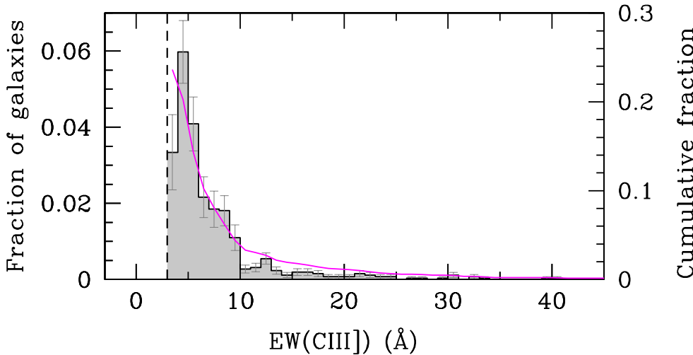
Fig. 7. Distribution of CIII]- \lambda 1908 equivalent width EW(CIII]) in the UV-selected star-forming population at 2 < z < 3.8 . The shaded histogram shows the fraction of galaxies with a given EW(CIII]) in bins of \delta EW = 1 \text{ \AA} (left Y-axis), with Poisson uncertainties from the population statistics indicated as error bars. The cumulative fraction of galaxies with EW(CIII]) above a given EW(CIII]) limit is drawn as the continuous magenta line (values on the right Y-axis), relative to the total population of SFGs at that redshift. About 24% of SFGs with 2 < z < 3.8 present CIII]- \lambda 1908 \text{\AA} emission with EW(CIII]) \geq 3 \text{ \AA} .
