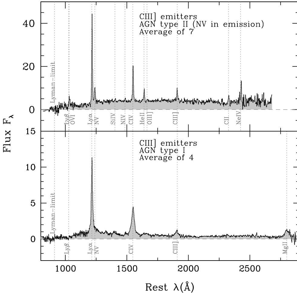
Fig. 14. Composite spectrum of four type I broad-line AGN ( bottom panel ), and seven candidate type II narrow-line AGN identified from their NV- \lambda 1240 emission ( top panel ). See text for details on how these AGN are selected.
