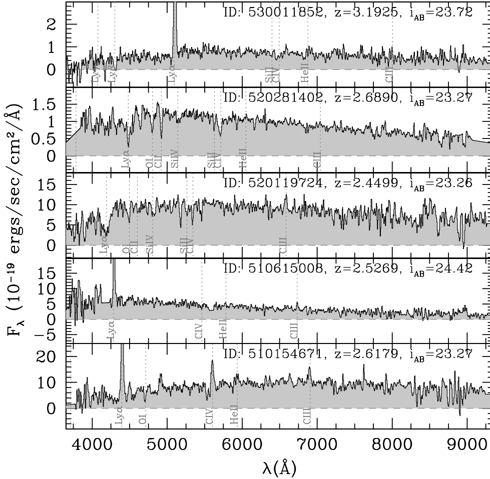
Fig. 3. Example VUDS spectra of weak CIII]1908 emitters with 0 < \text{EW}(\text{CIII])} < 5 \text{ \AA} .
