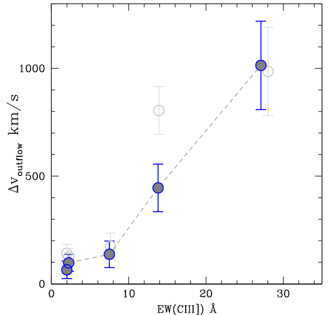
Fig. 10. Outflow velocity of ISM lines as a function of EW(CIII)] (filled symbols: velocity from the median values of the ISM lines; open symbols: mean values).
