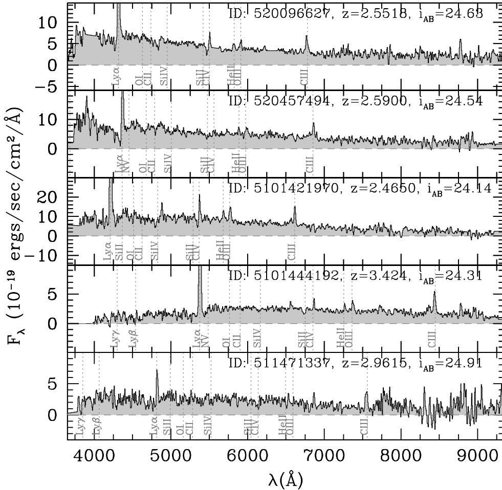
Fig. 2. Example VUDS spectra of strong CIII]1908 emitters with 10 < \text{EW}(\text{CIII])} < 20 \text{ \AA} .
