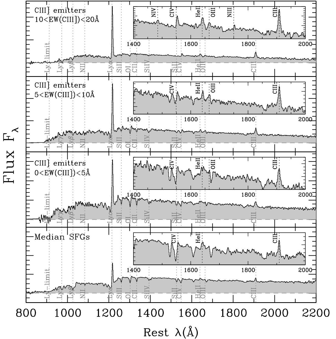
Fig. 4. Composite spectra of CIII]1908 emitters identified in the VUDS survey at 2 < z < 3.8 . From top to bottom: stack of 43 emitters with 10 < \text{EW}(\text{CIII])} < 20 , 31 emitters with 5 < \text{EW}(\text{CIII])} < 10 , 30 emitters with 0 < \text{EW}(\text{CIII])} < 5 , and for comparison, a stack of 450 galaxies that are representative of the general SFG population in the redshift range 2.8 < z < 3.8 .
