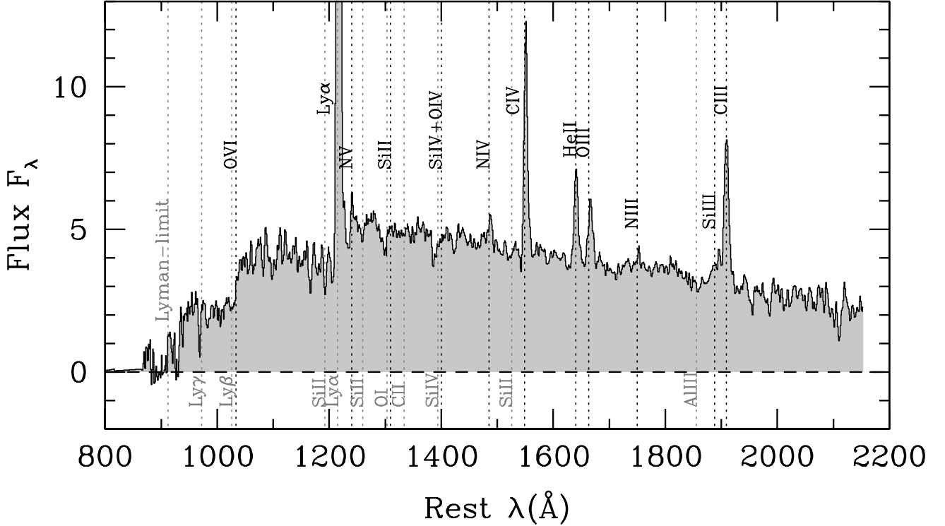
Fig. 5. Composite spectrum of 16 CIII]- \lambda 1908 emitters identified in the VUDS survey at 2 < z < 3.8 , where CIII] is detected in emission with S/N > 5 and EW(CIII)] > 20 Å. The main emission lines associated with CIII]- \lambda 1908 emission can be identified as Ly \alpha , NV- \lambda 1240, NIV]- \lambda 1485, CIV- \lambda 1549, HeII- \lambda 1640, OIII]- \lambda 1663, NIII]- \lambda 1750, and SiIII]- \lambda 1888.
