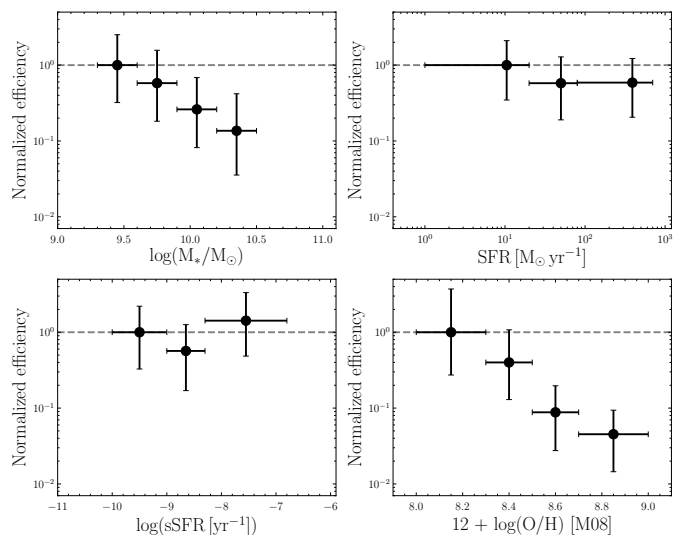
Fig. 3: The normalised efficiency of LGRB hosts compared to the MOSDEF sample at 1 < z < 2 as a function of stellar mass (top left panel), SFR (top right panel), sSFR (bottom left panel) and metallicity (bottom right panel). The values are normalized to the first bin. The horizontal grey dashed line indicates a value of 1 to guide the eye.
