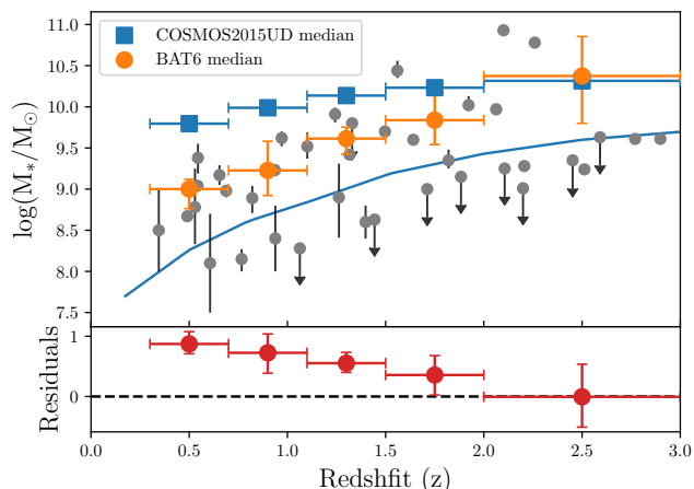
Fig. 4: Top panel: Stellar mass as a function of redshift. The grey circles are the individual host galaxies of the BAT6 sample; the orange circles represent the median stellar mass at each redshift bin for hosts above the COSMOS2015UD mass completeness. The blue squares represent the median of the SFR-weighted stellar mass distribution of the COSMOS2015UD sample at each redshift bin. The blue line is the mass completeness of the COSMOS2015UD sample. Bottom panel: Residuals of the difference between the blue and orange points. The errors are computed using Monte Carlo propagation and bootstrapping.
