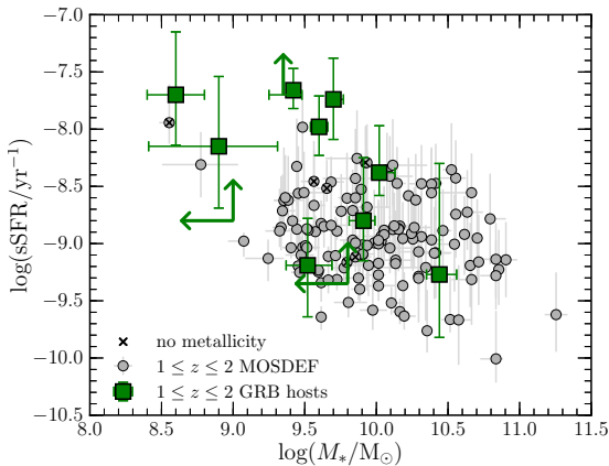
Fig. 8: sSFR versus stellar mass plot for the BAT6 sample at 1 < z < 2 . The grey circles are from the MOSDEF sample at 1 < z < 2 .
