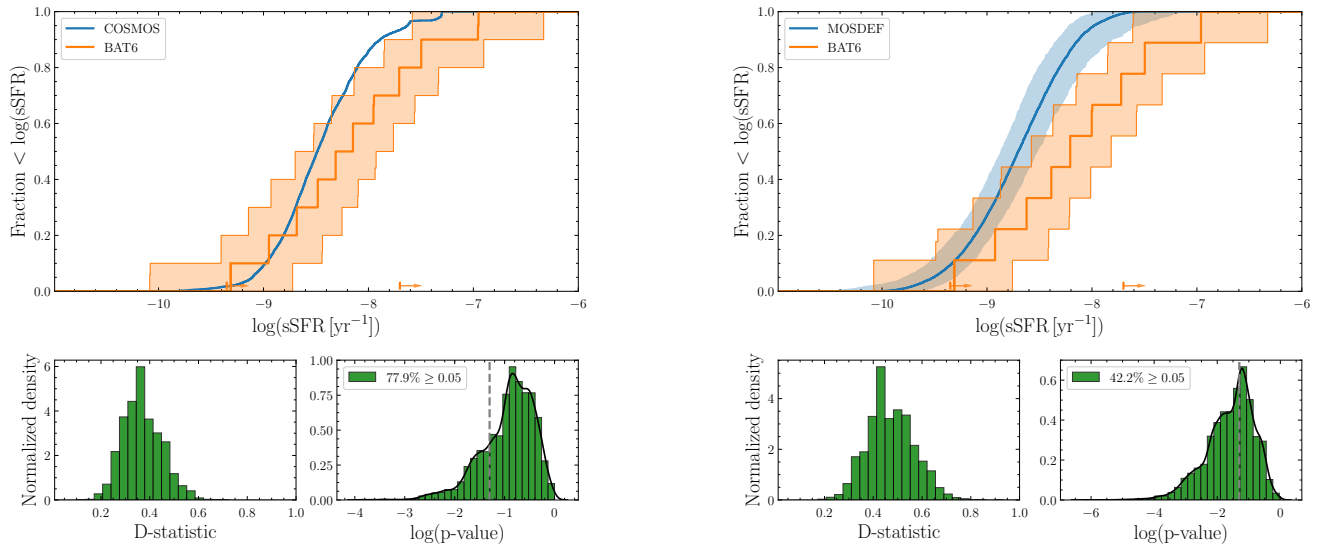
Fig. 6: Top panels: Cumulative sSFR distribution for the hosts of the BAT6 sample (orange) and the star-forming galaxies from the COSMOS2015 Ultra Deep catalog (blue, left panel) and MOSDEF (blue, right panel) at 1 < z < 2 . The COSMOS2015 Ultra Deep and MOSDEF CDFs are weighted by SFR. Limits are indicated by arrows at the bottom of the plot. Bottom panels: See Fig. 2.
