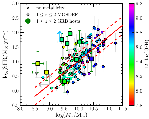
Fig. 7: SFR versus stellar mass plot for the BAT6 sample at 1 < z < 2 (squares). The circles are from the MOSDEF sample at 1 < z < 2 . The red line is the best fit to the MOSDEF data and the dotted lines represent the intrinsic scatter, following the method of Shivaei et al. (2015). The points are coloured by metallicity in the M08 calibrator. Galaxies where no metallicity could be measured are coloured in grey with a cross.
