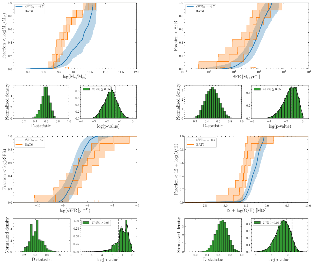
Fig. 14: The result of the same analysis as presented in Section 3 except using a sSFR cut on the MOSDEF sample of \log(\text{sSFR} [\text{yr}^{-1}]) = -8.7 .
