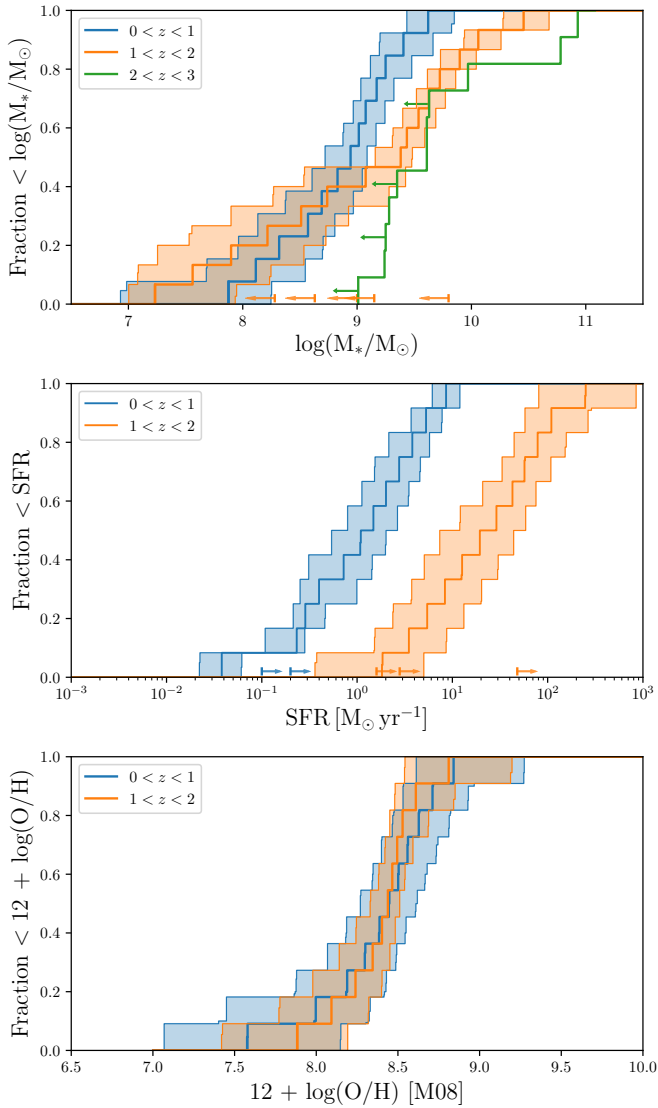
Fig. 1: Cumulative distributions of stellar mass (upper panel), SFR (middle panel) and metallicity (bottom panel) for the hosts of the BAT6 sample at different redshift ranges. Upper and lower limits are represented as arrows at the bottom of the plots. The shaded area represents the 95% confidence interval around the CDFs. The methodology to create these CDFs is presented in Sect. 3.2
