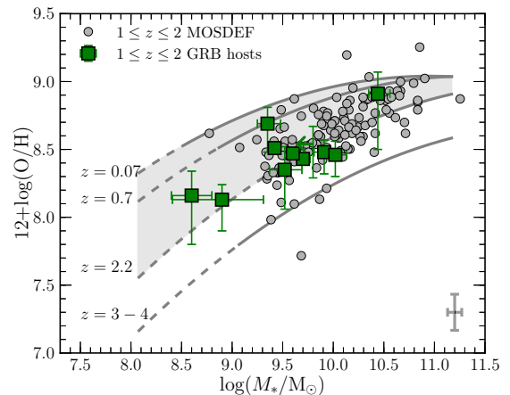
Fig. 10: MZR in the M08 calibrator for the BAT6 sample at 1 < z < 2 (squares). The grey points are from the MOSDEF sample at 1 < z < 2 , with their average uncertainty shown on the bottom right. The curves represent the MZR relation of Mannucci et al. (2009) from z = 0.07 to z \sim 3.5 , with the extrapolation below the mass completeness indicated in dashed.
