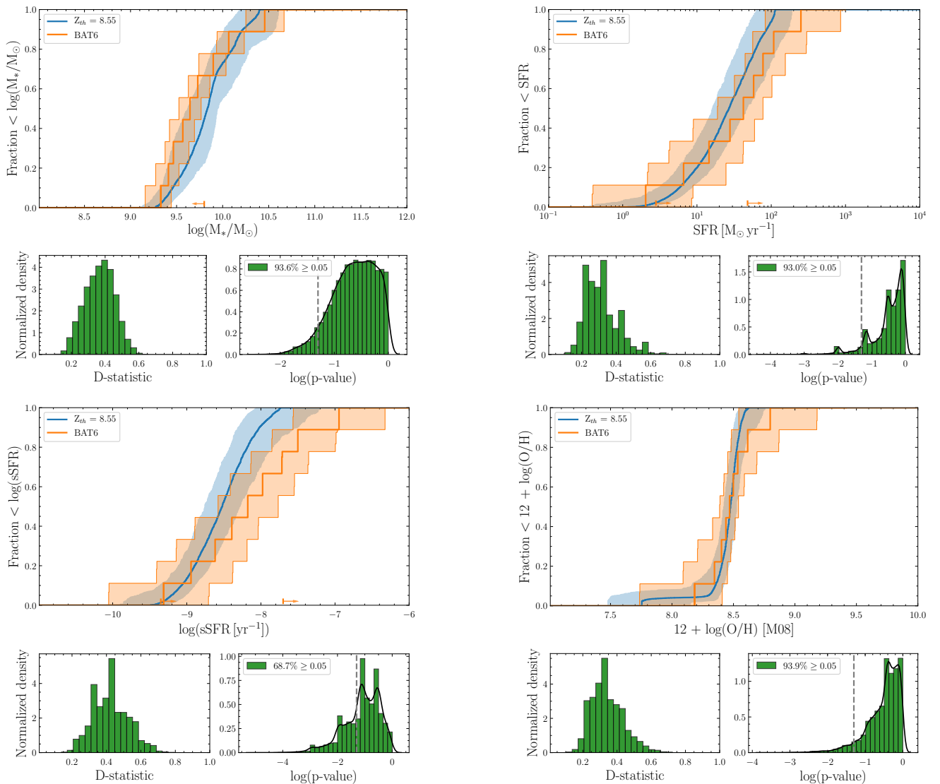
Fig. 13: The result of the same analysis as presented in Section 3 except using a metallicity cut on the MOSDEF sample of 12 + \log(\text{O}/\text{H})=8.55 . The CDFs match more closely, and the 2 sample K-S tests suggest we can not discard the null hypothesis in the majority of realisations.
