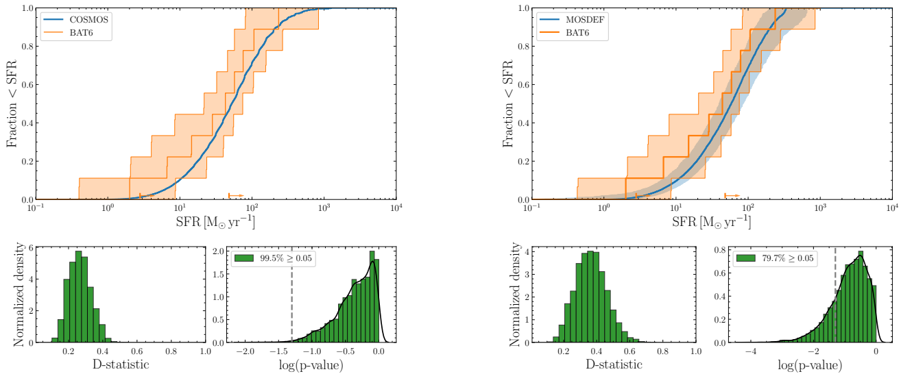
Fig. 5: Top panels: Cumulative SFR distribution for the hosts of the BAT6 sample (orange) and the star-forming galaxies from the COSMOS2015 Ultra Deep catalog (blue, left panel) and MOSDEF (blue, right panel) at 1 < z < 2 . The COSMOS2015 Ultra Deep and MOSDEF CDFs are weighted by SFR. Limits are indicated by arrows at the bottom of the plot. Bottom panels: See Fig. 2.
