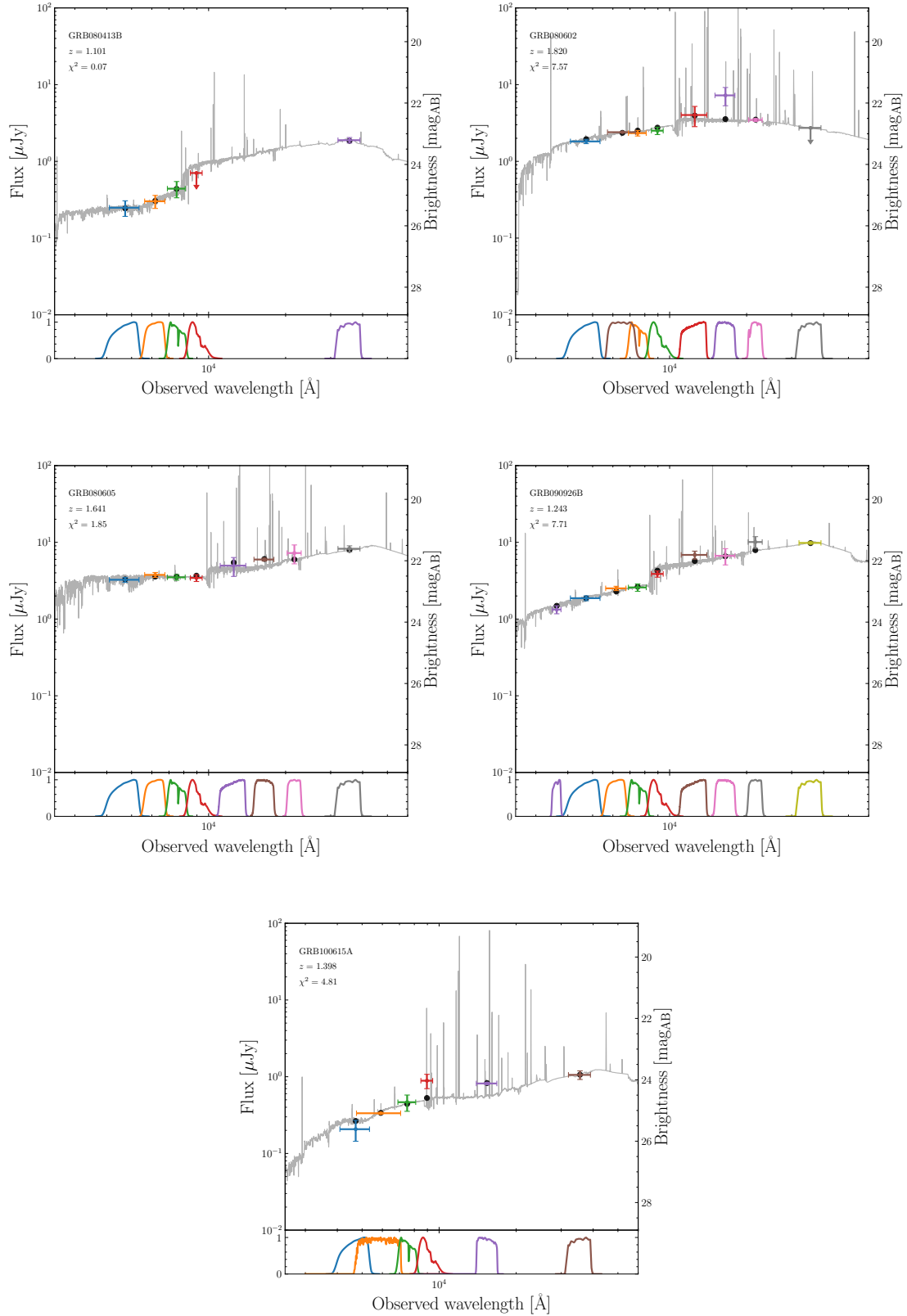
Fig. A.3: Same as Fig A.2
