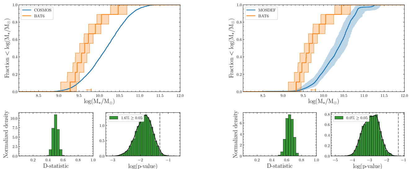
Fig. 2: Top panels: Cumulative stellar mass distribution for the hosts of the BAT6 sample (orange) and the star-forming galaxies from the COSMOS2015 Ultra Deep catalog (blue, left panel) and MOSDEF (blue, right panel) at 1 < z < 2 . The COSMOS2015 Ultra Deep and MOSDEF CDFs are weighted by SFR. Limits are indicated by arrows at the bottom of the plot. Bottom panels: Normalized histogram of the maximum distance between the BAT6 and the survey CDFs for each Monte Carlo realisation and of the p-value from the two-sample K-S test computed for each Monte Carlo realisation. The black curve represents the Gaussian kernel density estimation. The vertical dashed line indicates a p-value of 0.05, above which it is no longer possible to reject the null hypothesis that the two samples are drawn from the same distribution at a 95% confidence level.
