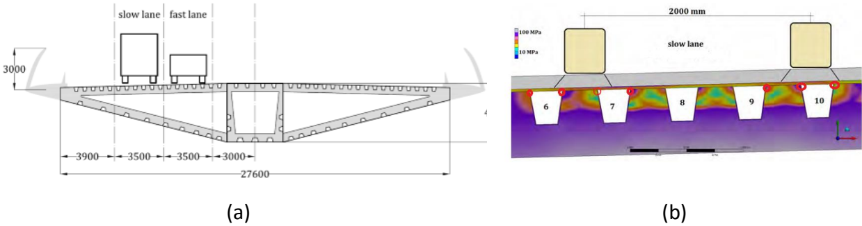
Figure 4: Cross-section of the deck of the Millau Bridge : (a) Whole cross-section, and (b) focus on the considered welds under the wheel loads of the heavy trucks on the slow lane.
