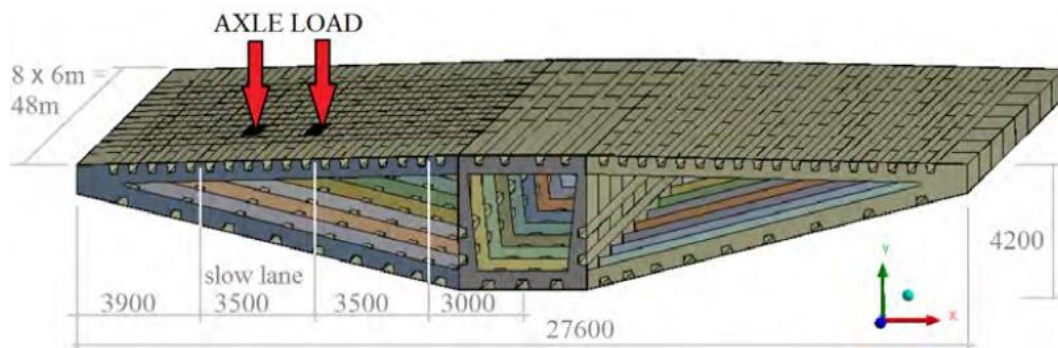
Figure 5: Geometry for the FE model analyzed with ANSYS software.
