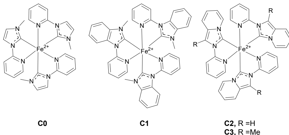
Figure1. Complexes studied in this work. Counter ion is PF 6 - in every case
