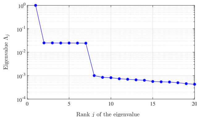
Figure 4: Eigenvalues of [p] for N_{\text{ir}} = 224 and \varepsilon_{\text{diff}} = 20 .
