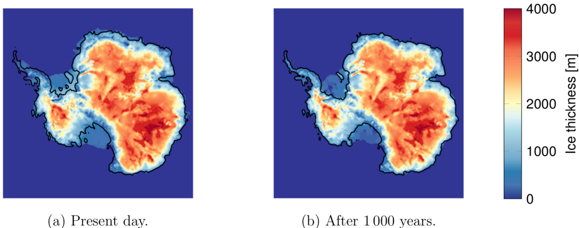
Figure 1: Ice thickness [m] (a) at present day and (b) after 1000 years obtained with nominal values of input variables.
