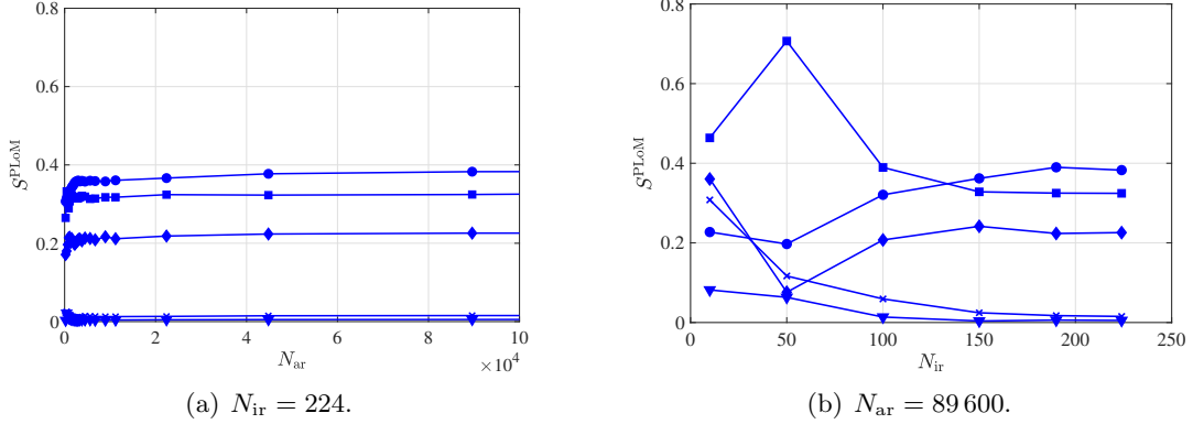
Figure 5: Estimates of the main-effect global sensitivity indices for the first (circle), second (square), third (diamond), fourth (triangle), and fifth (x-mark) uncertain input variables obtained by using the PLoM method (a) as a function of N_{\text{ar}} for N_{\text{ir}} = 224 and (b) as a function of N_{\text{ir}} for N_{\text{ar}} = 89600 . For the values of N_{\text{ir}} different from 224, the values of n_{\text{MC}} are different from 400.
