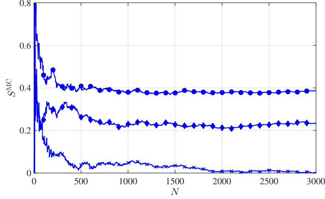
Figure 2: Estimates of the main-effect global sensitivity indices for the first (circle), third (diamond), and fifth (x-mark) uncertain input variables obtained by using the Monte Carlo method as a function of N .
