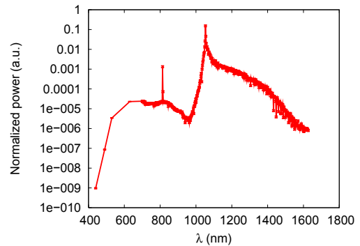
Figure 2. Spectrum emitted by the supercontinuum source.
