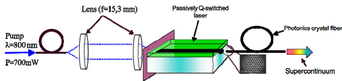
Figure 1. Schematic view of the supercontinuum source.
