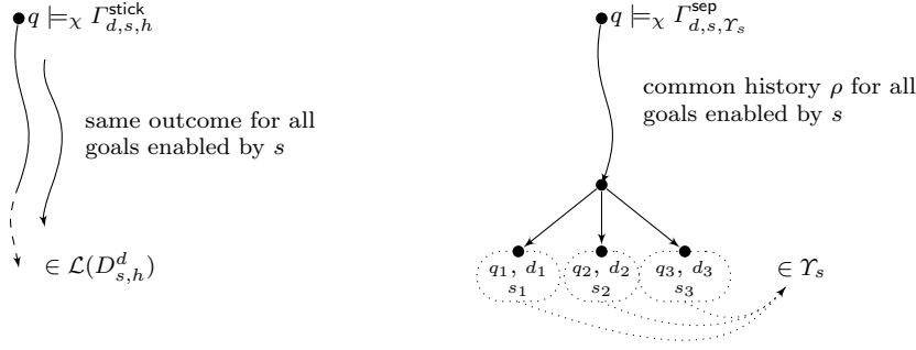
Fig. 9 Illustration of \Gamma_{d,s,h}^{\text{stick}} and \Gamma_{d,s,Y_s}^{\text{sep}}
