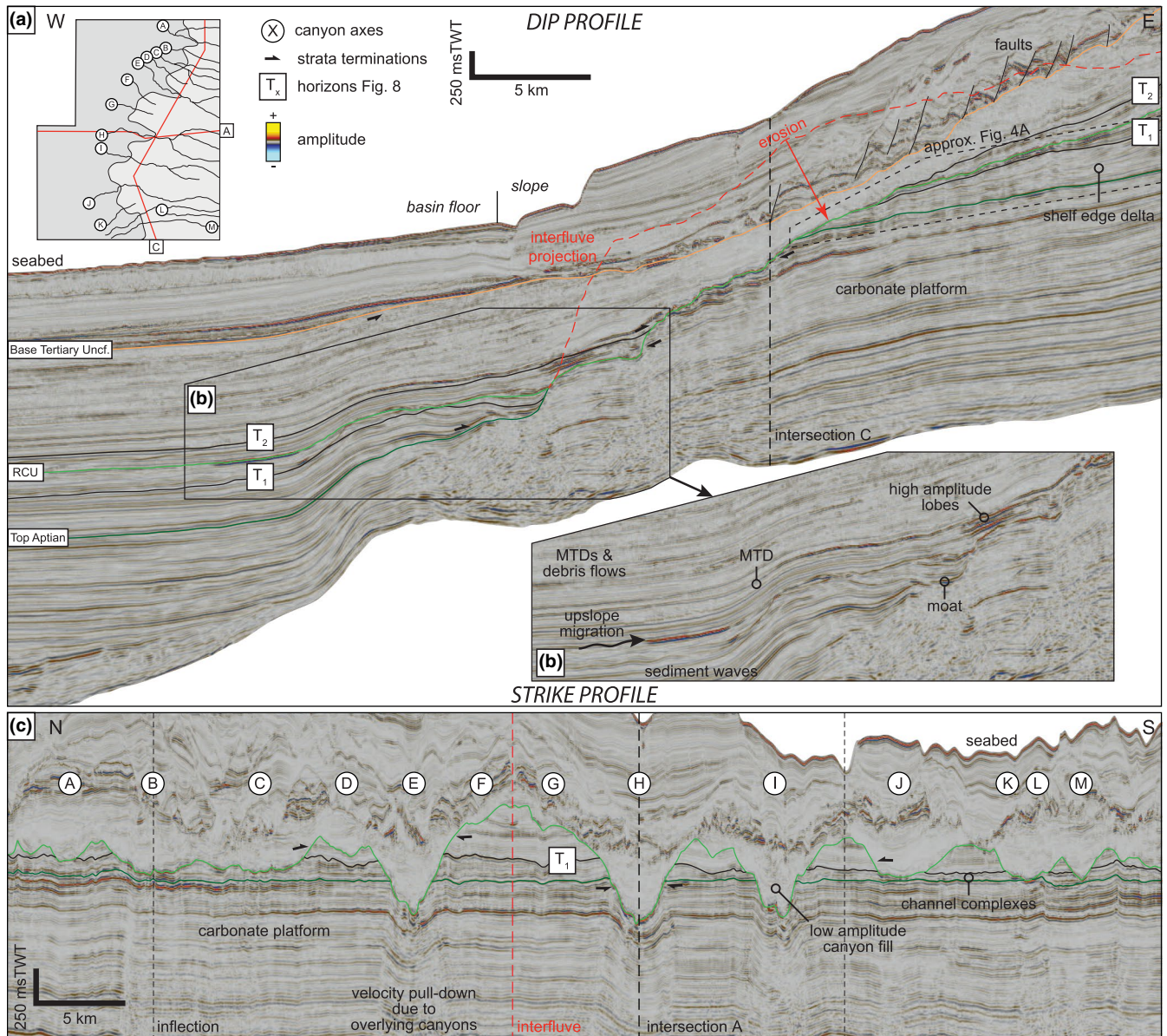
FIGURE 3 (a) East-West two-way time seismic section with interpreted key stratigraphic surfaces. The regional composite unconformity (RCU) surface on the adjacent interfluve is projected onto the dip profile (dashed red line) highlighting the amount of erosion in canyon H. Intersections shown in (c). (b) Inset seismic section focusing on seismic facies identified at the base of the canyon, MTD, mass transport deposit. (c) North-South two-way time seismic section with canyon axes displayed. See inset map (a) for the line locations. Seismic data courtesy of TGS
