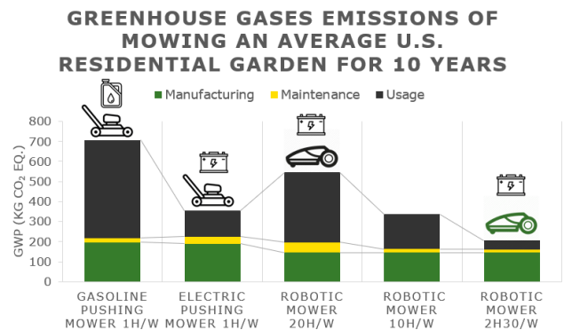
Fig. 3. Quantitative results of the LCA: bar charts, with icons
