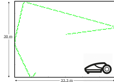
Fig. 2. Simulations to estimate the mowing time for 0.25 acre, random walk
