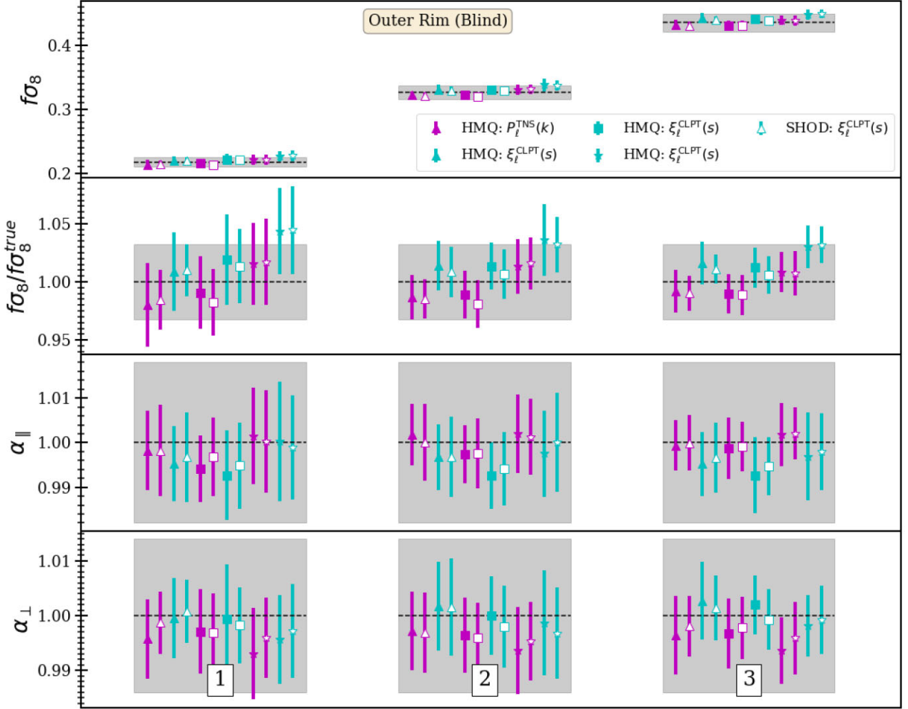
Figure 5. Results of RSD fits to the OUTER RIM blind mocks. From top to bottom, the four panels present the parameters f\sigma_8 , f\sigma_8/f\sigma_8^{\text{true}} , \alpha_{\parallel} , and \alpha_{\perp} . The x-axis shows the three different blind models with the triangle, the square, and the star marker for RSD realizations along x -, y -, and z -axes, respectively (see Table 8 for values). The magenta and cyan points correspond to the TNS and CLPT models, respectively. The filled and empty points correspond to the HMQ and SHOD models for ELGs. The error bars correspond to the 1\sigma measurement uncertainty. The black-dashed lines show the true value of these parameters with the grey-shaded region showing the systematic error proposed in this work. It is clear from the top panel that our choice of blind mocks cover a wide range of growth rate which is consistently recovered by the two RSD models.
