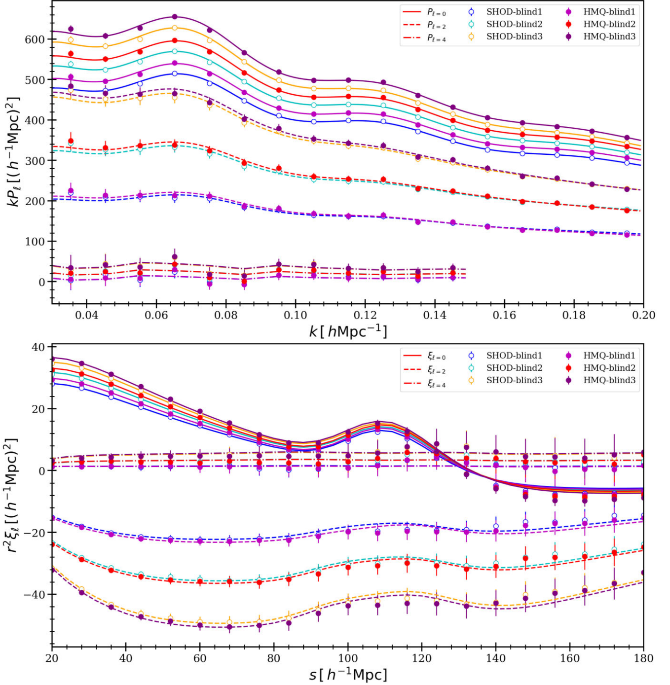
Figure 6. Clustering measurement for the blind mocks along with the best-fitting models. The top panel shows the power spectrum multipoles and the bottom panel the correlation function multipoles. The measurements from the mocks along with their error are shown with the circles, whereas the best-fitting models are shown with the lines. The mocks from the model with quenching (i.e. HMQ) are shown with the filled symbols and those from the model without quenching (i.e. SHOD) are shown with the empty symbols. The solid, dashed, and dot-dashed lines are for the Legendre moments with \ell = 0 , \ell = 2 , and \ell = 4 respectively. The power spectrum uses TNS, whereas the correlation function uses CLPT–GSRSD to model the redshift space distortions. Both models describe the mocks remarkably successfully.
