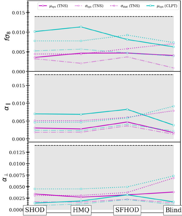
Figure 7. Comparison of systematic and statistical absolute errors for f\sigma_8 (top), \alpha_{\parallel} (middle), and \alpha_{\perp} (bottom). The x-axis shows the results for different kind of mocks. In each panel, the solid line is for \mu_{\text{sys}} representing mean systematic shift, the dot-dashed line is for \sigma_{\text{sys}} representing the rms of mean systematic shift from true values of the parameter, and the dashed line is for \sigma_{\text{stat}} representing statistical errors. The magenta colour is for the TNS model and the cyan colour for CLPT. The shaded region with the black-dashed line shows the theoretical systematic error proposed in this work. We note that a detection of systematic bias as per our definition will mean that the coloured solid lines above twice the value of the corresponding coloured dashed lines. Therefore, this figure illustrates that for both RSD model and all four type of mock catalogues we do not detect any systematic bias.
