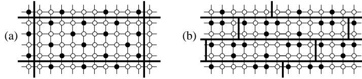
Fig. 6.6 Black vertices are the elements of a periodic code in G_S , which is (a) 1-LD with density \frac{3}{10} , (b) 1-Id with density \frac{7}{20} .
