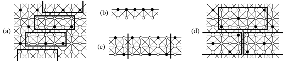
Fig. 6.9 Black vertices are the elements of a periodic code which is (a) 1-LD with density \frac{1}{5} in G_K , (b) 1-LD with density \frac{1}{2} in G_K^{[2]} , (c) 1-LD with density \frac{4}{15} in G_K^{[3]} , (d) 1-Id with density \frac{2}{9} in G_K .
