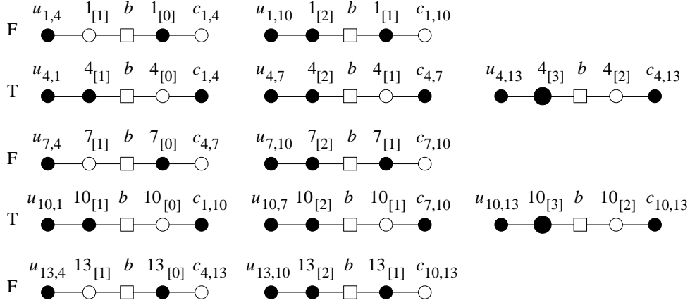
Figure 4: In black, the codewords in the 12 gadgets from Example 12, with x_1 = \text{F} , i.e., \ell_1 = \text{F} , \ell_4 = \text{T} , \ell_7 = \text{F} , \ell_{10} = \text{T} , \ell_{13} = \text{F} .
