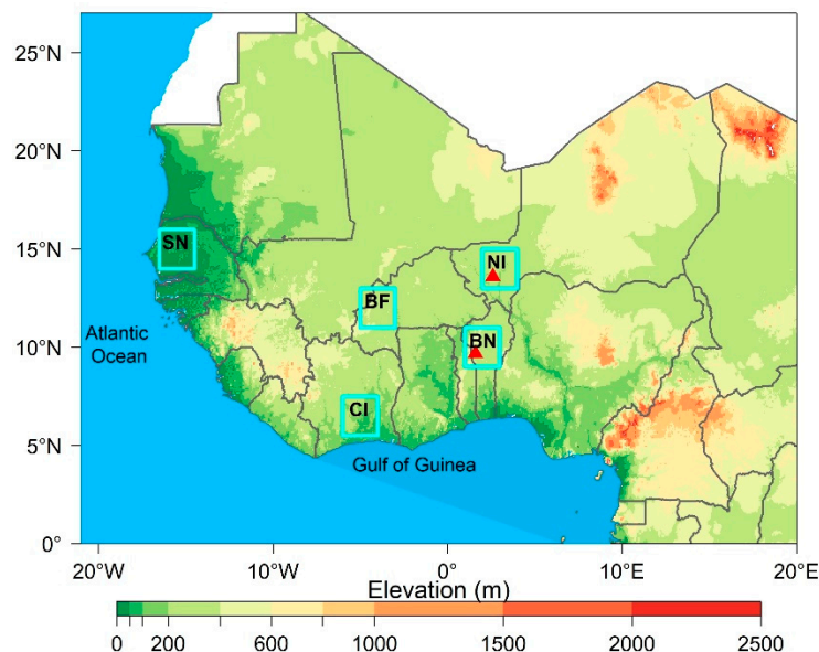
Figure 1. Elevation map of West Africa showing five 2^\circ \times 2^\circ boxes across the region in Senegal (SN), Burkina Faso (BF), Niger (NI), Benin (BN, and part of Togo), and Cote d’Ivoire (CI). The map also shows the locations of the two AMMA-CATCH (African Monsoon Multidisciplinary Analysis—Couplage de l’Atmosphère Tropicale et du Cycle eco-Hydrologique) observatories in Benin and Niger (red triangles).
