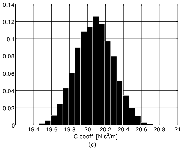
Figure 1. Histograms of A , B and C coefficients for a normalized 1% dispersion of all parameters except n_{TC} , n_{PT} , n_B , n_P
