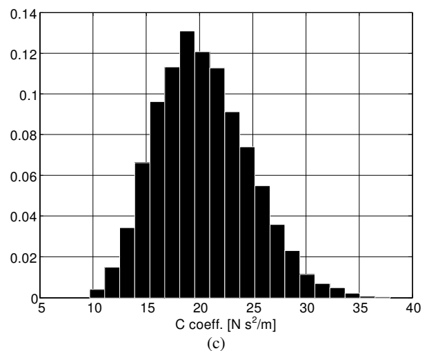
Figure 2. Histograms of A , B and C coefficients for a normalized 20% dispersion of all parameters including n_{TC} , n_{PT} , n_B , n_P
