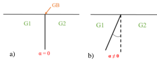
Figure 7: A schematic showing the GB plane a) perpendicular ( \alpha = 0 ), and b) inclined ( \alpha \neq 0 ) to the material free surface.
