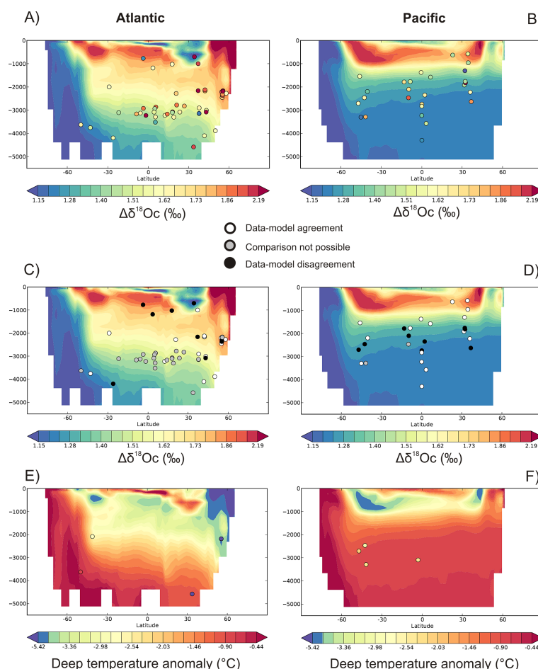
Figure 13. Atlantic and Pacific zonal mean anomaly (LGM-CT) for (a) Atlantic and (b) Pacific simulated deep ocean calcite \delta^{18}\text{O} in iLOVECLIM and global benthic foraminifera data (Table S2); (c) and (d) same as (a) and (b) but taking into account the uncertainties on calcite \delta^{18}\text{O} data ( 2\sigma ). Grey points (comparison not possible) denote the absence of error bars on data or denote locations where model results are not comparable to data (coastal sites). (e) and (f) Simulated deep temperature in iLOVECLIM and deep temperature reconstructions for the Atlantic and for the Pacific Oceans respectively (Adkins et al., 2002; Waelbroeck et al., 2002; Malone et al., 2004; Siddall et al., 2010; Elderfield et al., 2012). For colour scale generation explanations see Fig. 1 caption.
