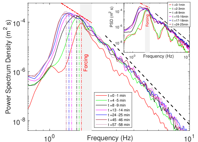
FIG. 2. Temporal evolution of the power spectrum density (PSD) of the wave height at x = 20 m (averaged on 4 probes n o 5, 10, 11, 12 - see Fig. 1). \sigma_\eta = 1.14 cm. Gray area: Forcing bandwidth. Dash-dotted vertical lines correspond to the maximum of each spectrum. Dash-dotted red line is the prediction in f^{-11/3} of Eq. (1). Dashed black line displays a f^{-6} fit. Inset: Same for x = 2 m (averaged on probes n o 1, 2).
