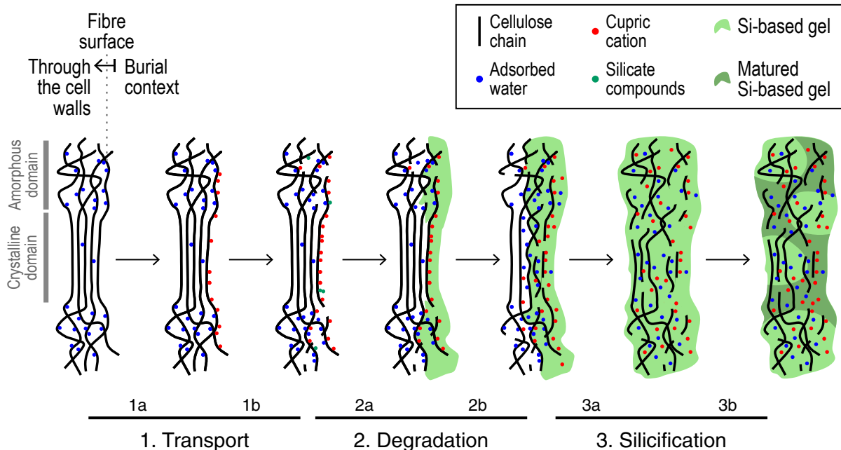
Fig. 5. Mechanism for cellulosic fiber mineralization over time. Step 1: Water transport of biocidal metal cations and soil solutes—formation of copper-cellulose complexes at the surface of the fibers (1a) and hydrolysis of amorphous compounds and condensation of silicates on fiber surface and in amorphous areas (1b). Step 2: Degradation and loss of crystallinity of cellulosic polysaccharides—degradation of the superficial macromolecules of the crystalline zones (2a) and local swelling (2b). Step 3: Silicification—diffusion of solutes deeper into the cell walls and condensation of siliceous compounds (3a) and maturation in denser siliceous phases (3b).
