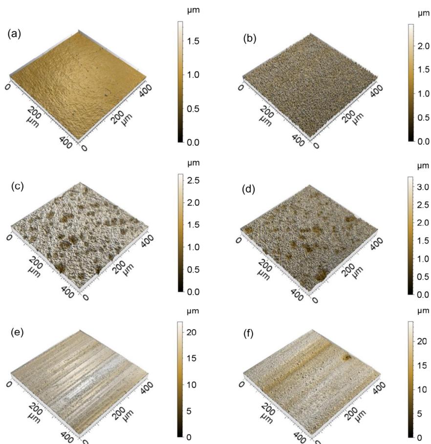
Fig. 7. 3D images reconstituted by profilometry in the case of (a) untreated PP, (b) treated PP, (c) untreated PE, (d) treated PE, (e) untreated PVC, and (f) treated PVC, for V_{\text{DBD}} = 30 kV, f = 800 Hz, square waveform, exposure time = 15 min.
