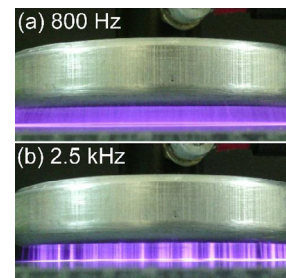
Fig. 2. Photography of the DBD for frequency of (a) 800 Hz and (b) 2.5 kHz; applied voltage amplitude: V_{DBD} = 30\ \text{kV} .
