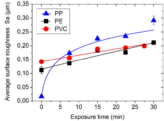
Fig. 6. Average surface roughness versus exposure time. (a) Polypropylene, (b) polyethylene, (c) polyvinyl chloride, for V_{\text{DBD}} = 30 kV, f = 800 Hz, square waveform.
