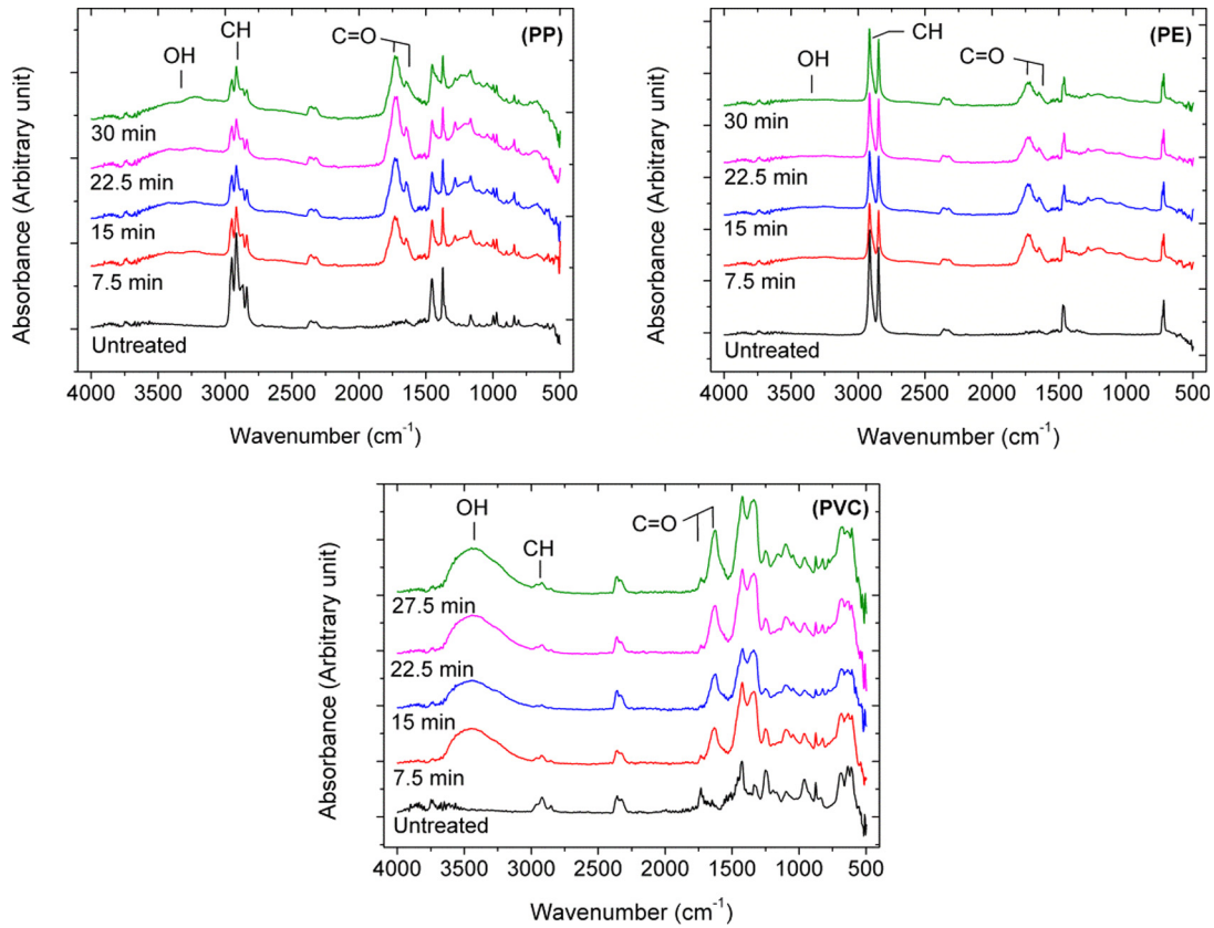
Fig. 8. FTIR spectrum changes versus exposure time. Conditions: V_{DBD} = 30 kV, f = 800 Hz, square waveform.
