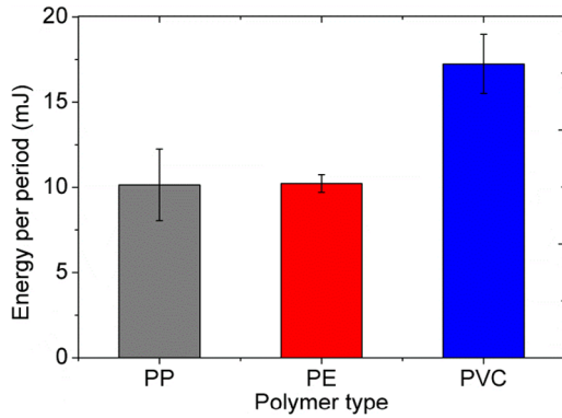
Fig. 5. DBD energy per period depending on the nature of treated polymer, for V_{\text{DBD}} = 30 kV, f = 800 Hz.
