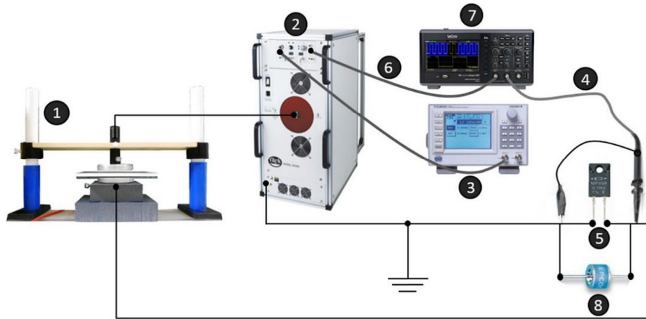
Fig. 1. The DBD experimental setup schematic representation. (1) DBD cell, (2) HV power amplifier, (3) function generator, (4) current measurement channel, (5) non-inductive resistor of 100\ \Omega , (6) voltage measurement channel, (7) oscilloscope, (8) spark gap protection.
