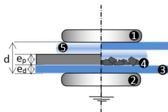
Fig. 3. Experimental setup for DBD treatment. (1) Active electrode, (2) grounded electrode, (3) dielectric barrier (glass), (4) polymer sample (granules or slab), (5) plasma.
