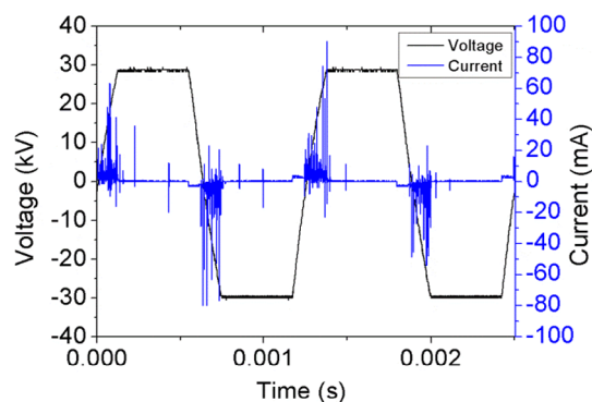
Fig. 4. Typical current and voltage waveforms of DBD, in the case of polypropylene treatment, V_{\text{DBD}} = 30 kV, f = 800 Hz.
