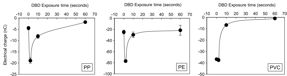
Fig. 9. Granules acquired tribo-charge variation versus DBD exposure time.
