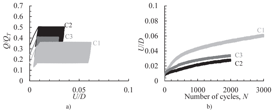
Figure 4. Results of tests C1, C2 and C3: (a) normalized cyclic load-displacement response; (b) displacement response with cycles.
