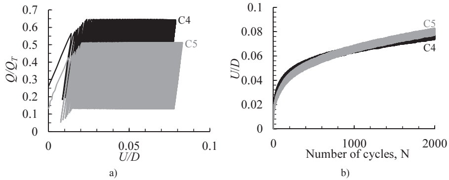
Figure 5. Results of tests C4 and 5 (a) normalized cyclic load-displacement response; (b) displacement response with cycles.
