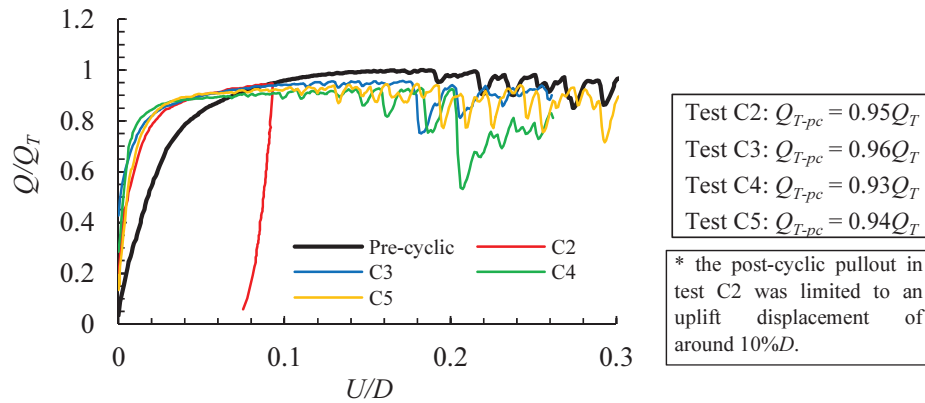
Figure 6. Pre-cyclic and post-cyclic monotonic load-displacement responses.
