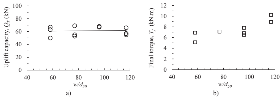
Figure 3. (a) Uplift capacity and (b) final installation torque of models of different sizes.
