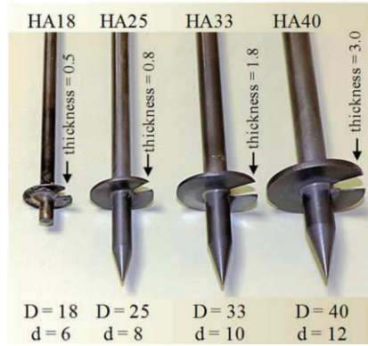
Figure 2. Helical anchor models (dimensions in mm).
