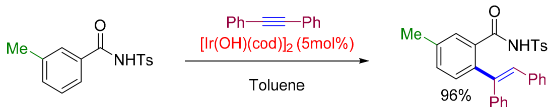
Scheme 3. Alkenylation of benzene.
