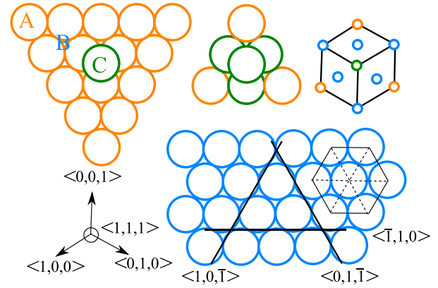
Fig. 1. FCC and slip directions in \langle 1, 1, 1 \rangle plane.
