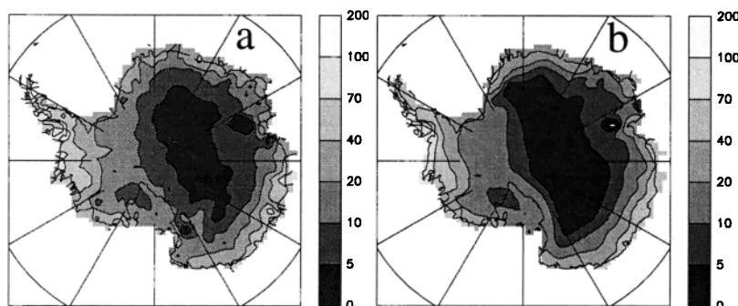
Figure 1. Mean SMB of Antarctica according to (a) Vaughan et al. [1999] and (b) Giovinetto and Bentley [1985]. Units are \text{cm yr}^{-1} .
