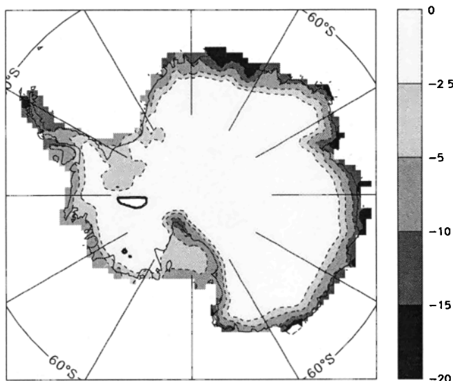
Figure 8. Model composite sublimation (water flux positive downward). Units are \text{cm yr}^{-1} .
