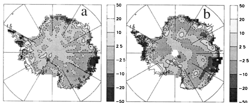
Figure 5. The reduced composite model SMB biases (see section 4.1) at (a) high and (b) low resolution. Negative contours are dashed. Units are cm yr -1 .
