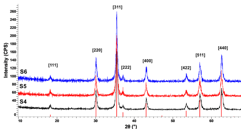
Figure 4. XRD patterns of samples synthesized at 200 °C.
