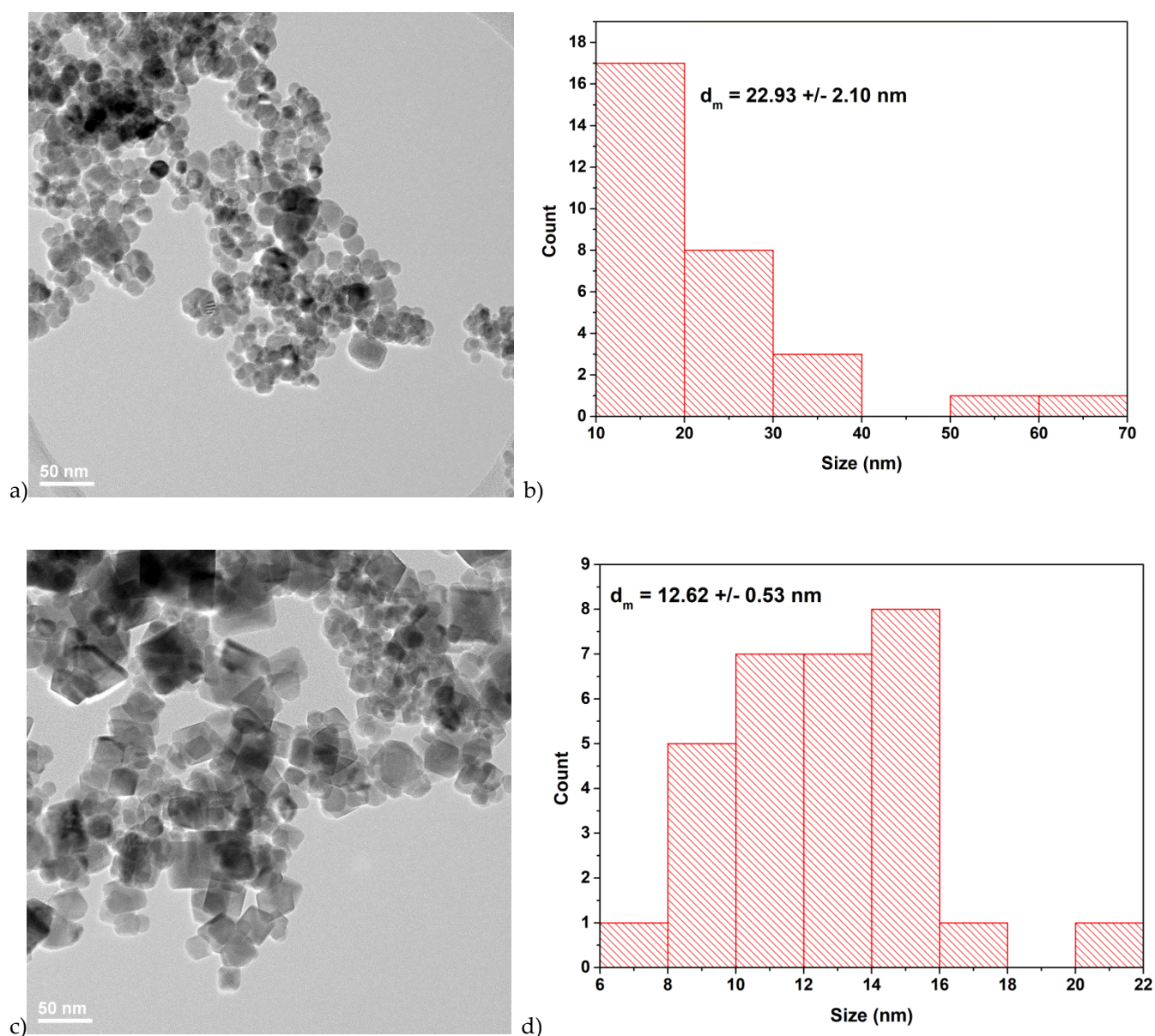
Figure 5. Transmission electron microscopy (TEM) images and core size distribution of samples: a) S3 (prepared at 100 °C/100 atm); b) size distribution of sample S3; c) S6 (prepared at 200 °C/100 atm); d) size distribution of sample S6.
