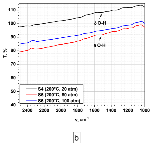
Figure 2. FT-IR analysis of samples prepared at 200 °C: a) wavenumber range. 4000–2500 cm -1 ; b) wavenumber range 2500–550 cm -1 .
