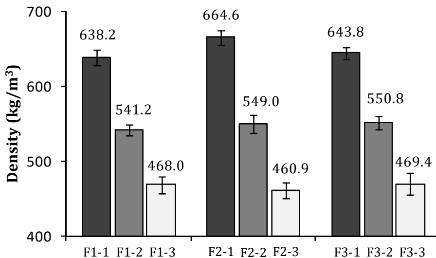
Figure 7. Density of the different formulations of flax concrete.
