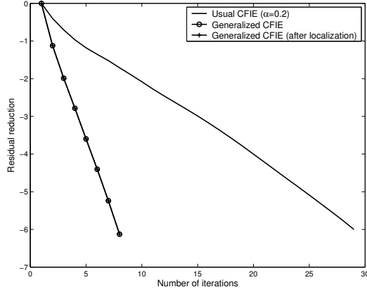
Fig. 19 History of the residual norm vs. the number of iterations for the unit sphere (for k = 35 ).
