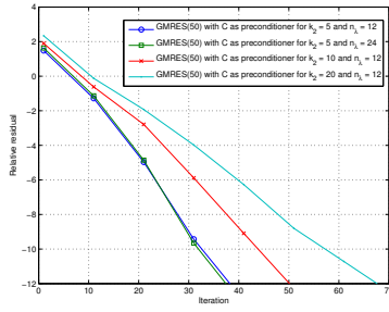
(a) Convergence history of GMRES(50) for the unit square cylinder.
