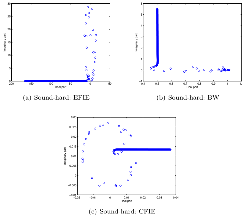
Fig. 10 Sound-hard spheres: distribution of the eigenvalues for the EFIE, BW and CFIE.
