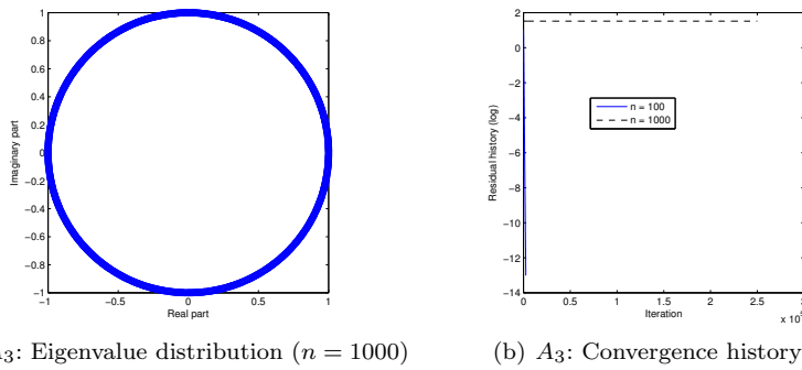
Fig. 3 Matrix A_3 .
