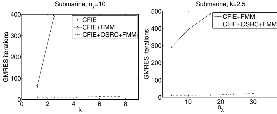
Fig. 18 Sound-hard submarine: number of GMRES iterations with respect to the wavenumber k (left) and the density n_\lambda (right).
