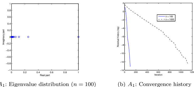
(a) A_1 : Eigenvalue distribution ( n = 100 )
