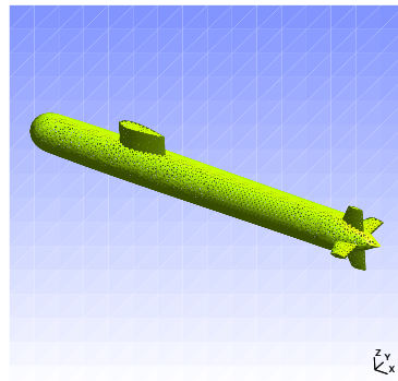
Fig. 16 A 3D realistic configuration: mesh of a submarine.
