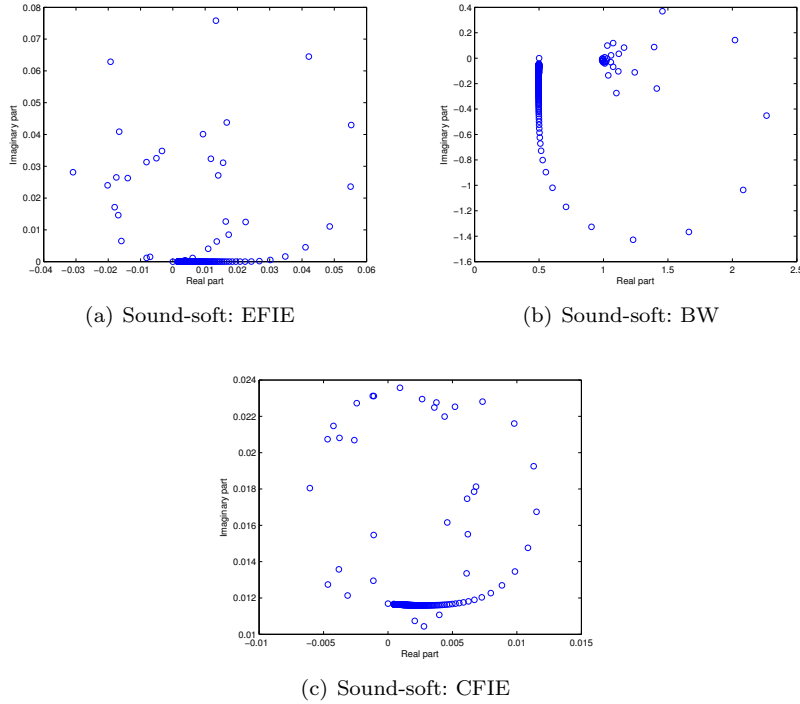
Fig. 9 Sound-soft sphere: distribution of the eigenvalues for the EFIE, BW and CFIE.
