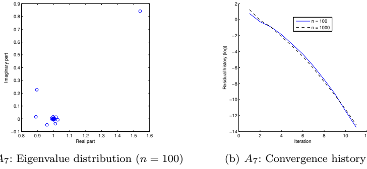
Fig. 6 Matrix A_7 .
