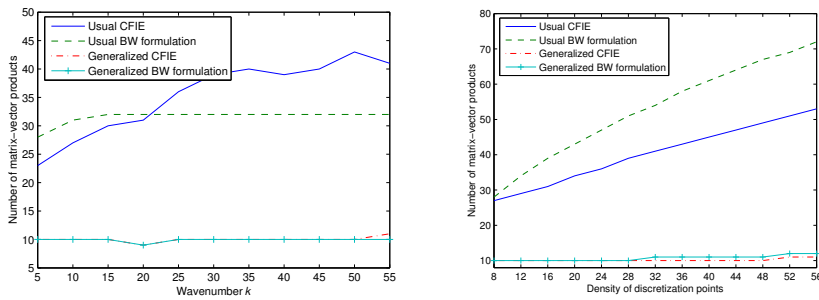
Fig. 14 Sound-hard unit square cylinder: number of MVPs for the four integral formulations with respect to the wavenumber k (left: n_\lambda = 10 ) and the density n_\lambda of discretization points per wavelength (right: k = 10 ).
