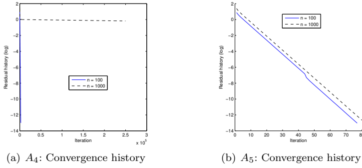
Fig. 4 Matrices A_4 and A_5 .
