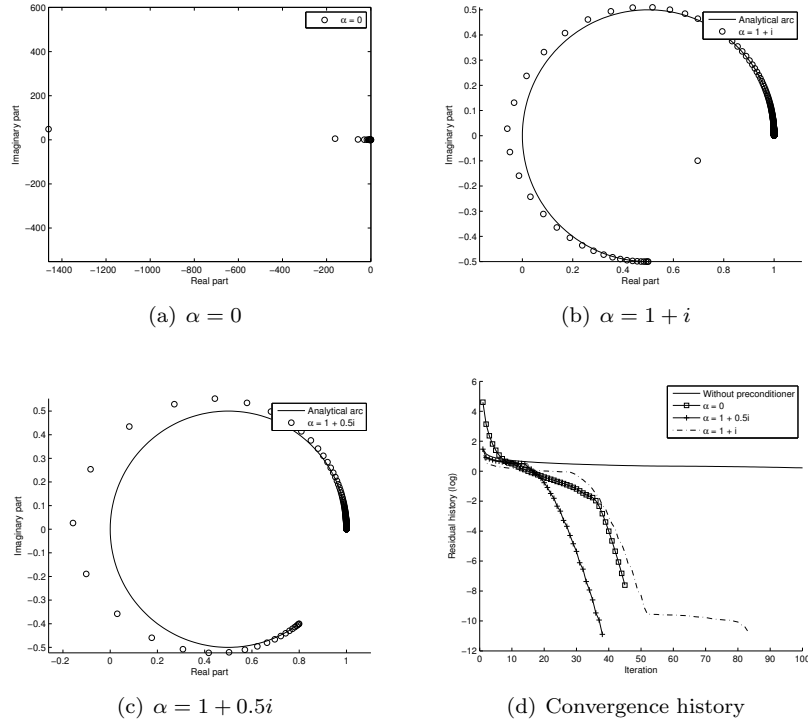
Fig. 8 Laplace shifted preconditioning.
