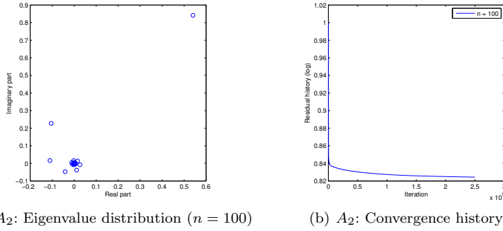
Fig. 2 Matrix A_2 .
