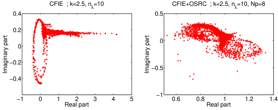
Fig. 17 Sound-hard submarine: distribution of the eigenvalues (left: standard CFIE, right: generalized CFIE), k = 2.5 , n_\lambda = 10 .
