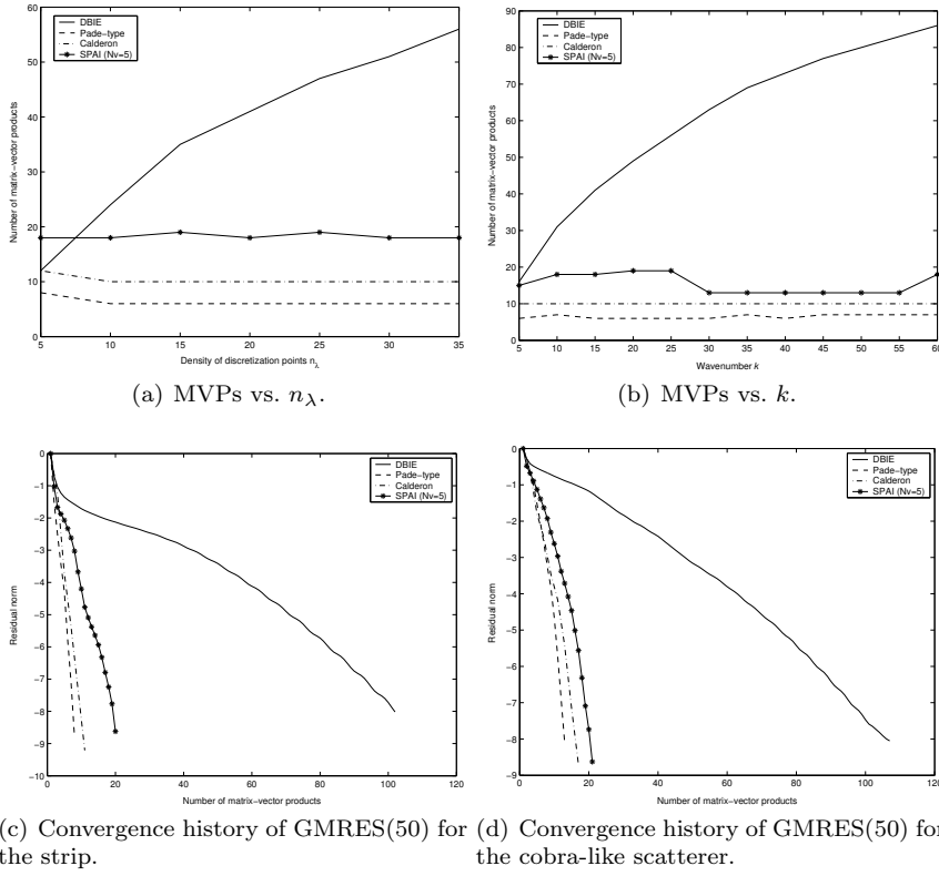
Fig. 12 Pseudodifferential preconditioner for scattering problems.
