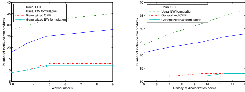
Fig. 15 Sound-hard ellipsoidal scatterer: number of MVPs for the four integral formulations with respect to the wavenumber k (left: n_\lambda = 10 ) and the density n_\lambda of discretization points per wavelength (right: k = 5 ).
