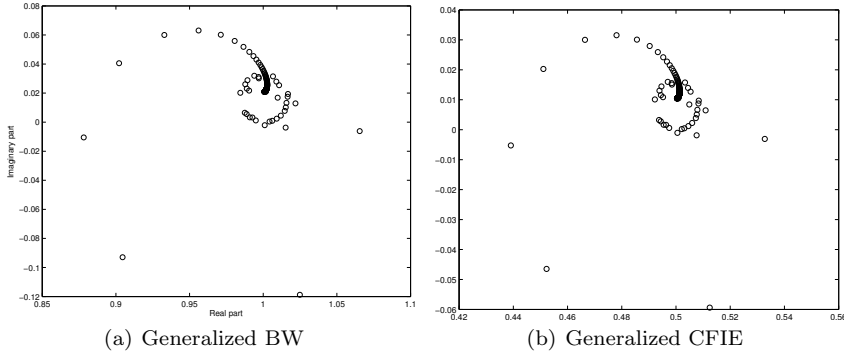
Fig. 13 Sound-hard sphere: distribution of the eigenvalues for the generalized combined field integral equations.
