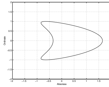
(b) The kite-shaped scatterer.
