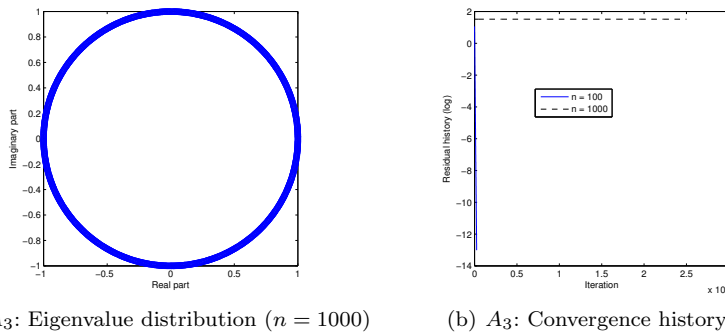
Fig. 3 Matrix A_3 .
