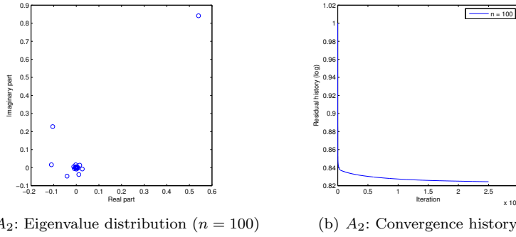
Fig. 2 Matrix A_2 .
