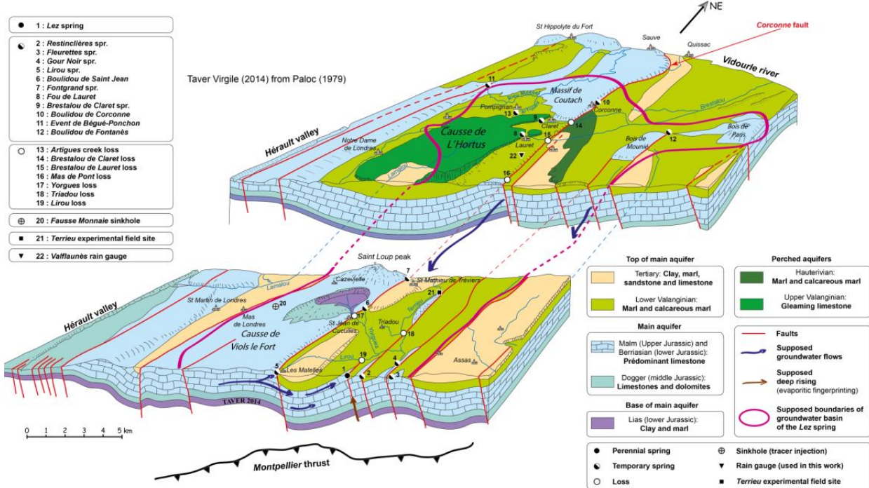
Interpretative diagram of the hydrogeological basin of the Lez spring (Taver, 2014 modified from Paloc, 1979)
