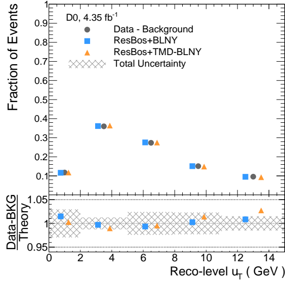
FIG. 3: [color online] Comparisons of the measured and predicted u_T distributions after the detector response simulation for different MC predictions based on RESBOS . The ratios of the background-subtracted data to each theory prediction are shown in the lower panel together with the 1\sigma uncertainty band. The total experimental uncertainty is indicated by the hatched band; it is dominated by the uncertainty due to the hadronic recoil calibration. The points for the predictions are offset horizontally to aid with visibility.
