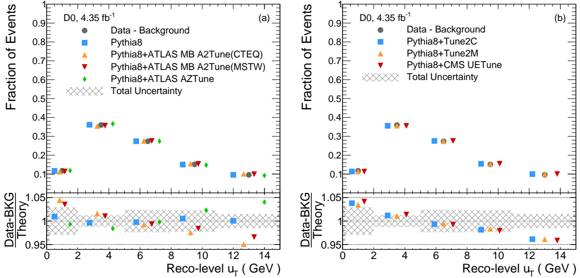
FIG. 4: [color online] Comparisons of the measured and predicted u_T distributions after the detector response simulation for different MC predictions based on PYTHIA . The ratios of the background-subtracted data to each theory prediction are shown in the lower panel together with the 1\sigma uncertainty band. The total experimental uncertainty is indicated by the hatched band; it is dominated by the uncertainty due to the hadronic recoil calibration. The points for the predictions are offset horizontally to aid with visibility.
